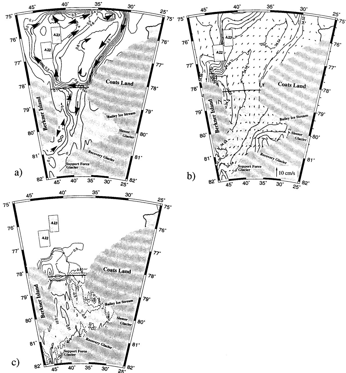
Figure 9. (a) Stream function for the vertically integrated mass transport (in Sv) for the postcalving scenario in 1995, when iceberg A24 has left the trough and the hydrographic measurements were obtained. Contour interval is 0.1 Sv below 0.5 Sv and 0.2 Sv above. (b) Bottom salinity distribution and bottom velocities (in \text{cm s}^{-1} ) for the same scenario. The northward shift of the icebergs leads to a slow increase of HSSW flow into the trough. (c) Fast ice extent (dotted line) as derived from the model results and freezing rate (in \text{m yr}^{-1} ; dashed lines indicate melting) of marine ice beneath and in front of the Filchner Ice Shelf.
