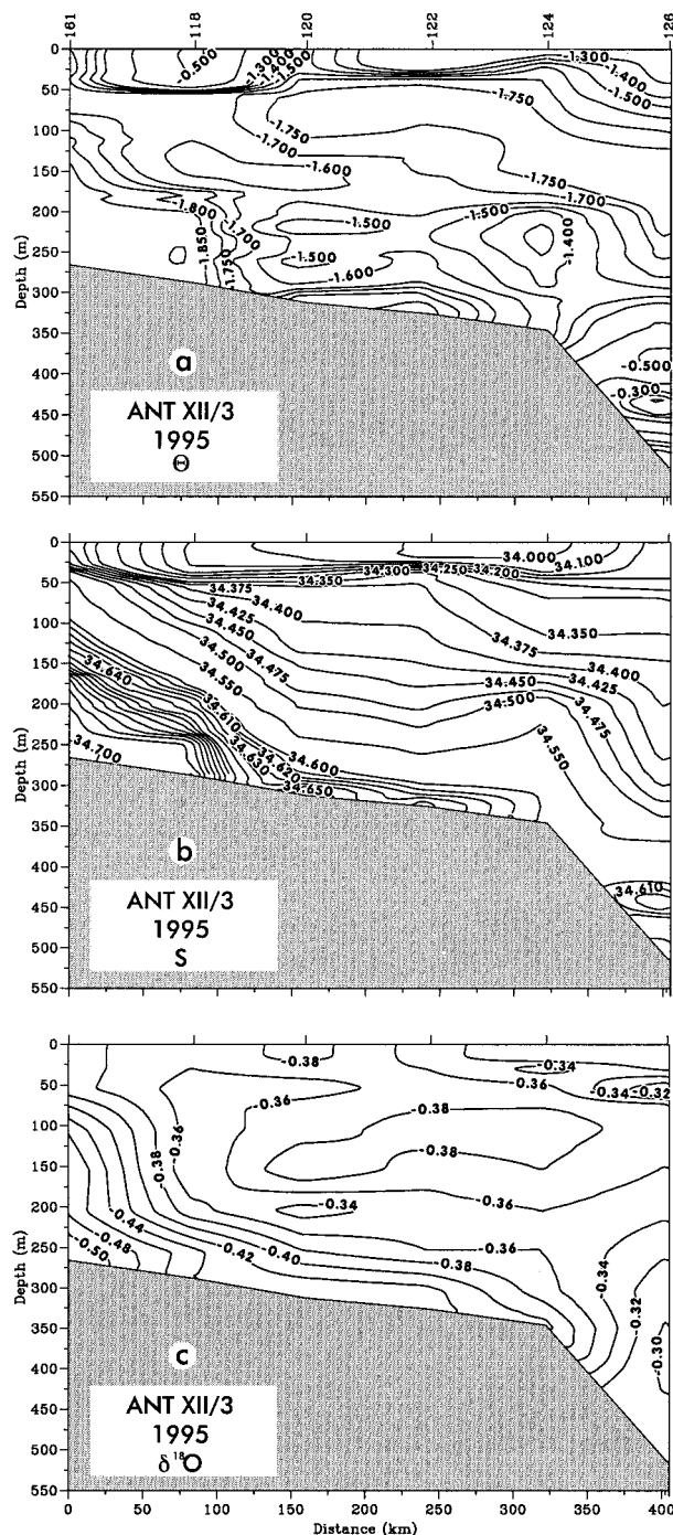
Figure 6. (a) Potential temperature, (b) salinity, and (c) \delta^{18}\text{O} of section 3 (Figure 3) from south to north across the Berkner Bank. Stations 161 and 118 depict the area where HSSW production occurs on Berkner Bank.
