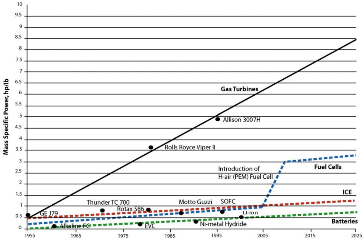
FIGURE 4.1-2: MASS SPECIFIC POWER TRENDS.
