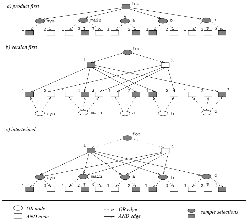
Fig. 7. Different kinds of AND/OR graphs and selection orders (I).
