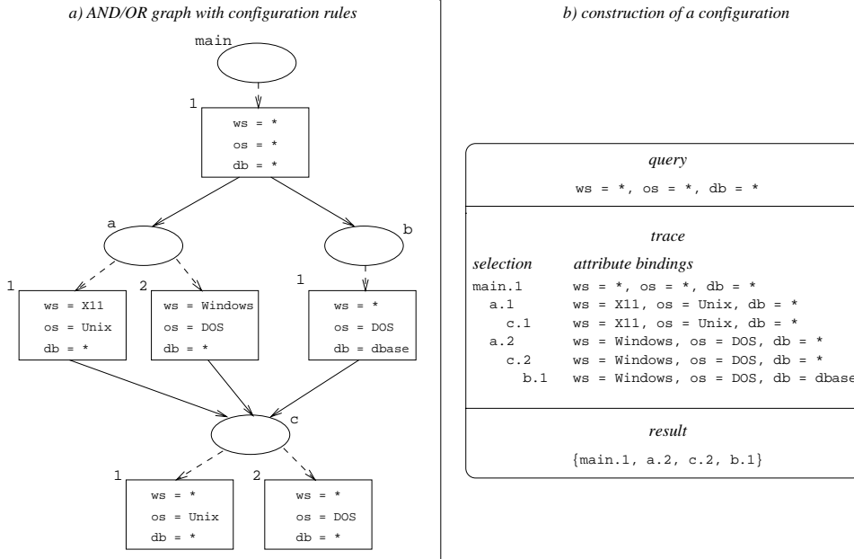
Fig. 18. Rule-based construction of a configuration.
