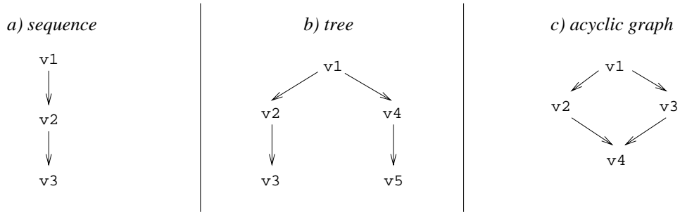
Fig. 3. Version graphs (one-level organization).
