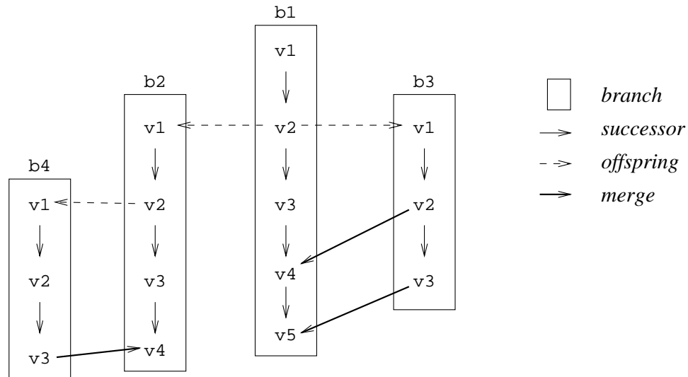
Fig. 4. Version graphs (two-level organization).
