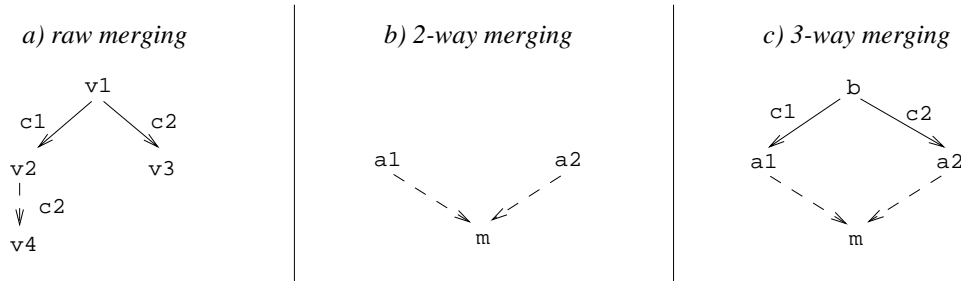
Fig. 19. Types of merging.
