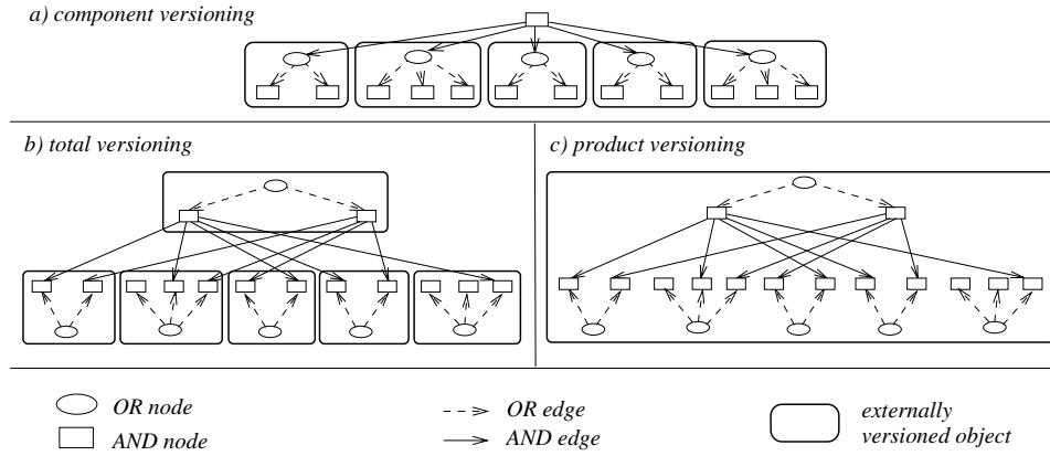
Fig. 9. External versioning.
