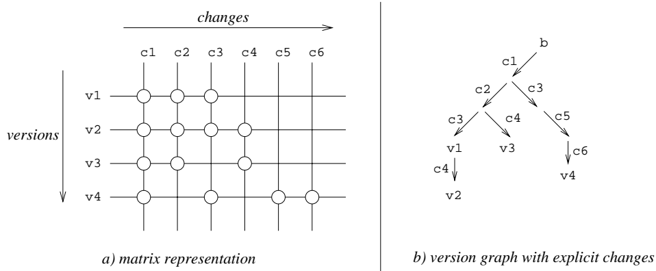
Fig. 6. Change space.
