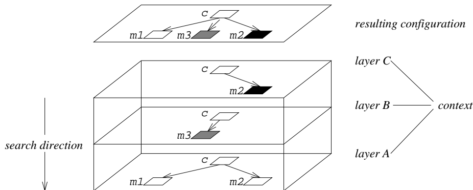
Fig. 21. Layers and contexts in PIE.
