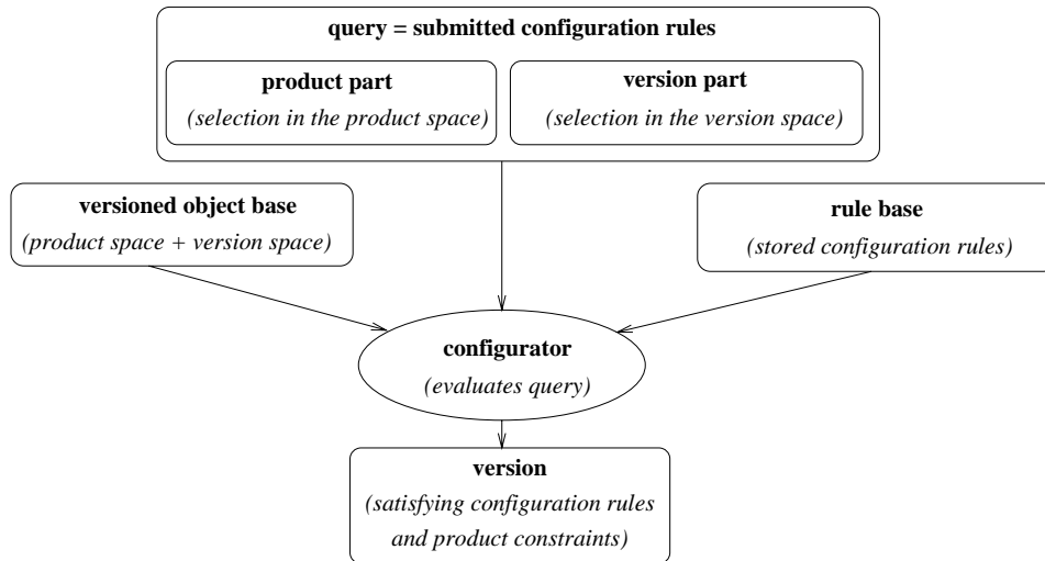
Fig. 14. Intensional versioning.
