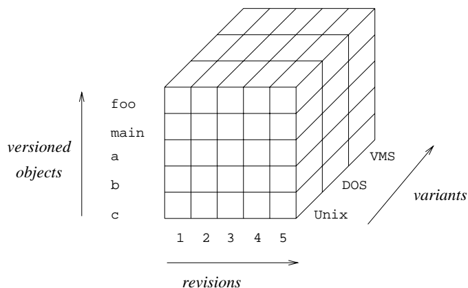
Fig. 11. Product versioning.
