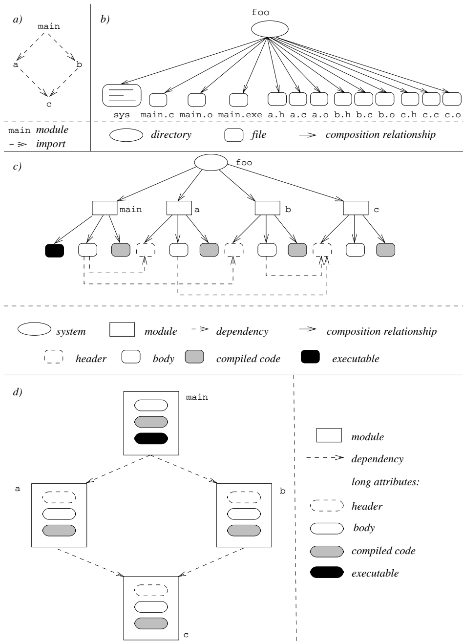
Fig. 1. Different representations of a software product.
