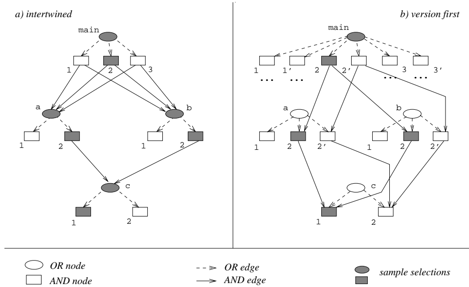
Fig. 8. Different kinds of AND/OR graphs and selection orders (II).
