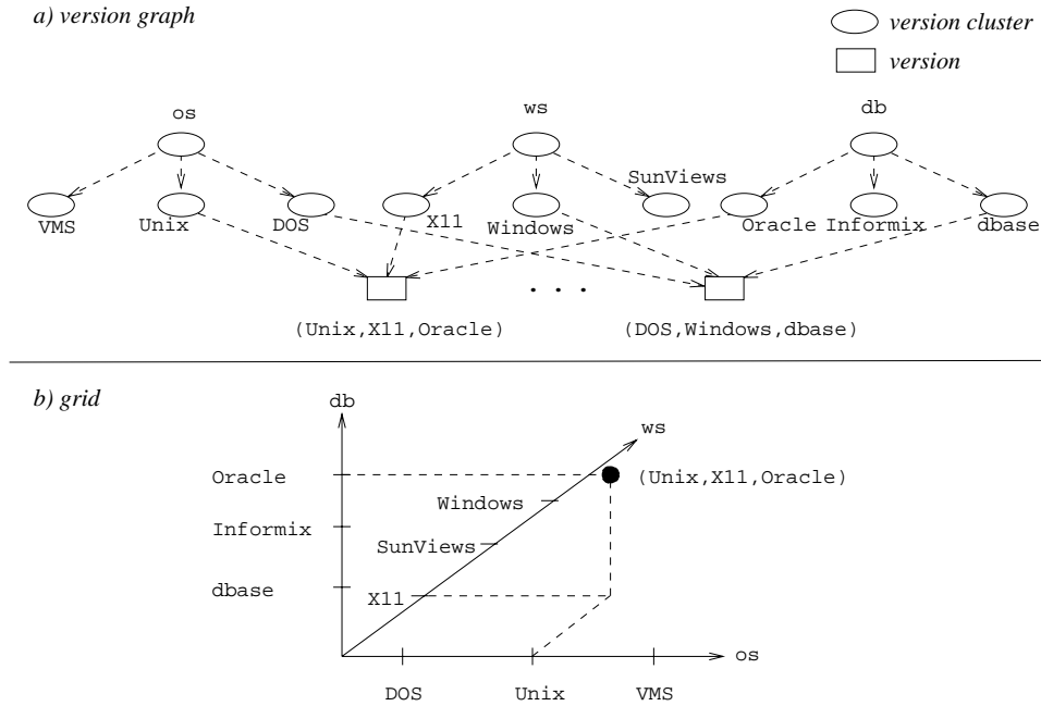
Fig. 5. n -dimensional variant space.
