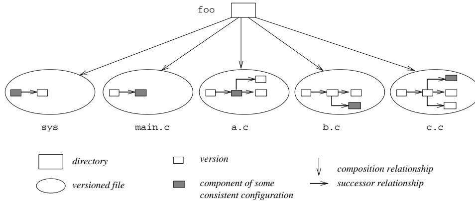
Fig. 10. AND/OR graph augmented with successor relationships.
