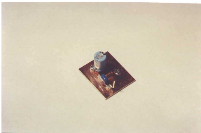
RF probe built Manhattan style.
