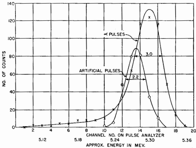
FIG. 6. Typical distributions of pulse sizes for polonium \alpha -particles and artificial pulses (Grid No. 1). One channel spacing on pulse analyzer is equal to 15 kev.
