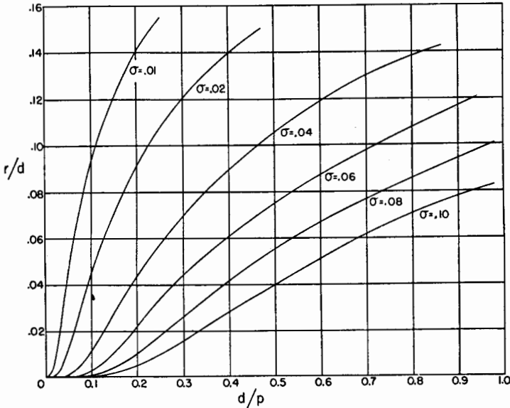
FIG. 3. Curves of constant inefficiencies \sigma of grids.
