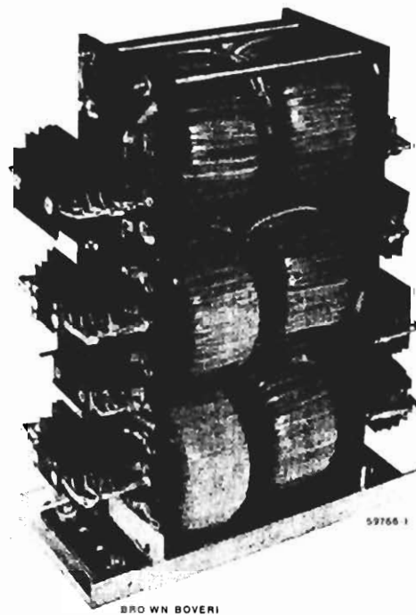
Fig. 1. — Band-pass filter for 2800–3200 cycle range.
