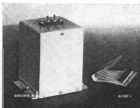
Fig. 5. — Matching unit with double-wire coils.
