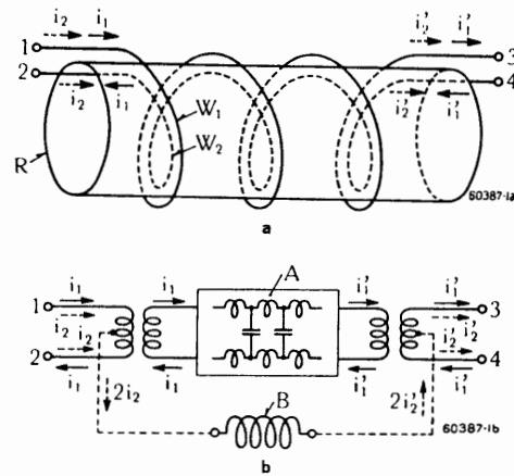
Figs. 1a and 1b. — Double-wire coil system with equivalent diagram.
