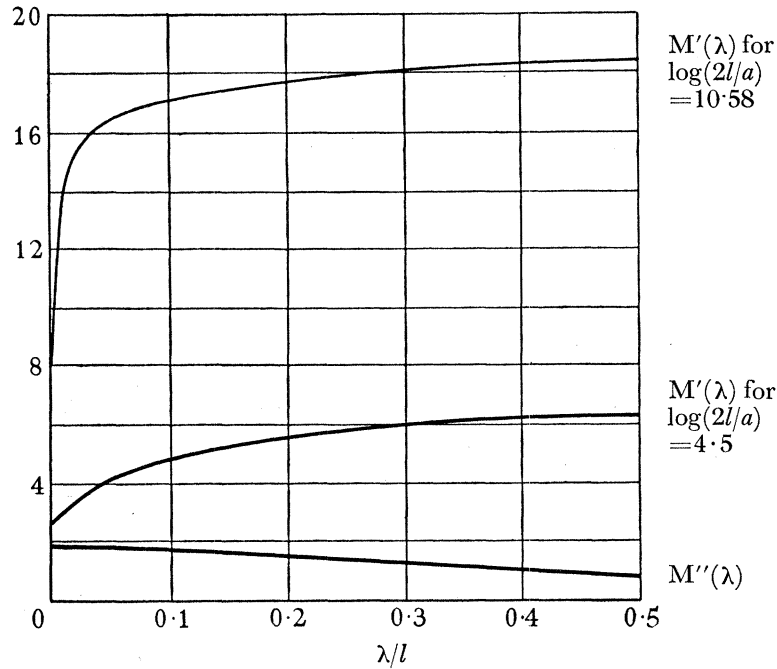
FIG. 3—Graph of the Function M(\lambda) = M'(\lambda) - iM''(\lambda) .—The upper curve drawn with a thin line is the graph of M'(\lambda) for \log(2l/a) = 10.58 and \alpha = 3.64 . The next curve represented by a thick line is the graph of M'(\lambda) for \log(2l/a) = 4.5 and \alpha = 3.64 . The lowest curve represents M''(\lambda) which is independent of \log(2l/a) . All the curves are symmetrical with respect to the point \lambda/l = 0.5 . To estimate the error involved by replacing 1/M(\lambda) by 1/\bar{M}(\alpha) in integrals involving \phi(\lambda) given by equation (20), we have determined by quadratures the mean value of 1/M(\lambda) in the interval 0 < \lambda < l as defined by
