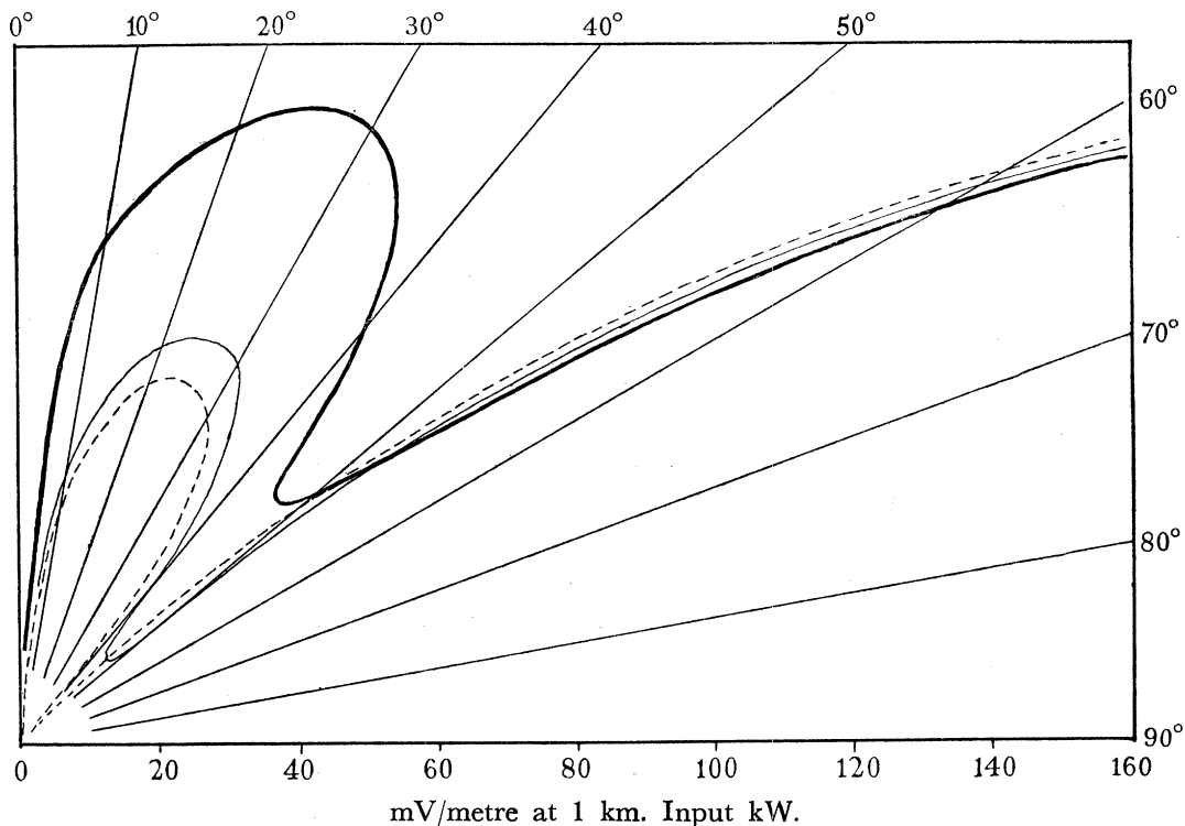
FIG. 7—Polar Diagram of Radiation Field—Enlarged part of the polar diagram of fig. 6 giving E_{\theta} l r.m.s. in millivolts per metre at 1 km. distance for 1 kW radiation output at \alpha = 3.64 . The thick curve corresponds to \log(2l/a) = 4.5 , the thin curve to \log(2l/a) = 10.58 , and the dotted curve to \log(2l/a) = \infty .
