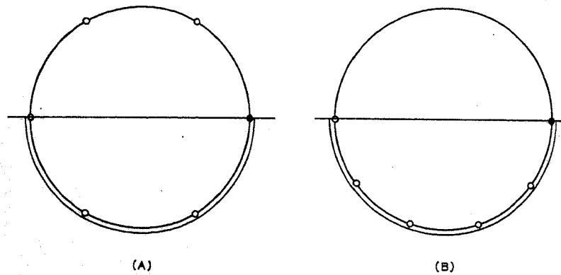
Fig. 14—Disposition of null points for the arrays with directive characteristics as shown in Fig. 13.
