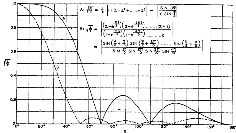
Fig. 13—Directive properties of 2 six-element arrays with \ell = \lambda/4 . Curve (A) refers to a uniform array and Curve (B) refers to an array with its nulls equispaced in the range of z .
