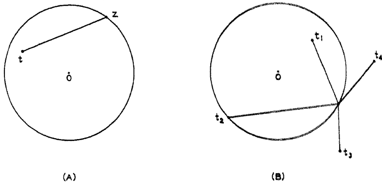
Fig. 7—The radiation intensity of a linear array is represented by the square of the product of the lines joining the null points of \sqrt{\Phi} to a point z on the unit circle.
