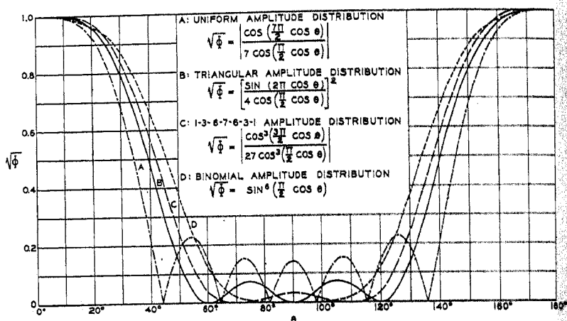
Fig. 5—Space Factors—(A) is for a uniform array and (B) for an array with "triangular" amplitude distribution.
