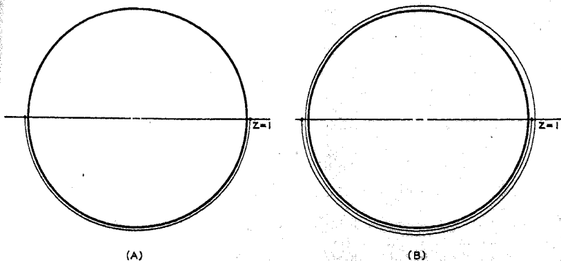
Fig. 3—(A) The active range of z , corresponding to \vartheta = \beta l and one-quarter wave-length separation between the elements. (B) The active range of z , corresponding to \vartheta = \beta l and l = \frac{1}{2}\lambda .
