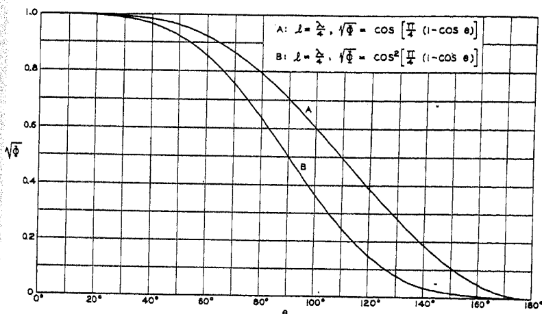
Fig. 4—Space Factors—Curve A is the space factor of a unidirectional couplet in which \lambda = \lambda/4 . Curve (B) represents the space factor of an array with amplitudes proportional to 1, 2, 1.
