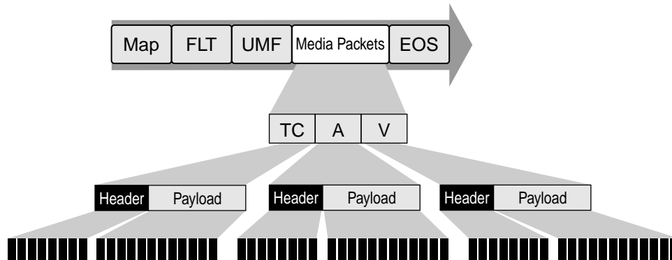
Figure 8 – Media packets
