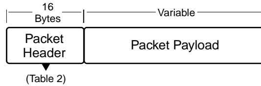
Figure 4 – Packet header
