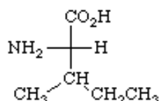
Isoleucine
