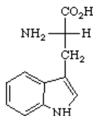
Tryptophan
