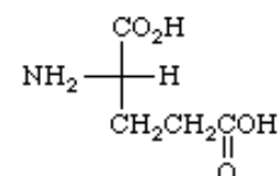
Glutamic Acid
