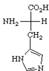
Histidine
