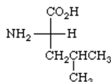
Leucine
