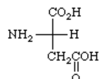
Aspartic Acid
