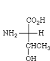
Threonine
