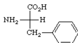
Phenylalanine
