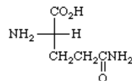
Glutamine
