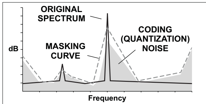
Figure A-3 Coding (Quantization) Noise Below the Masking Curve
