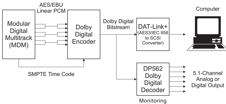
Figure 2-3 Dolby Digital Recorded to a Computer with DAT-Link+
