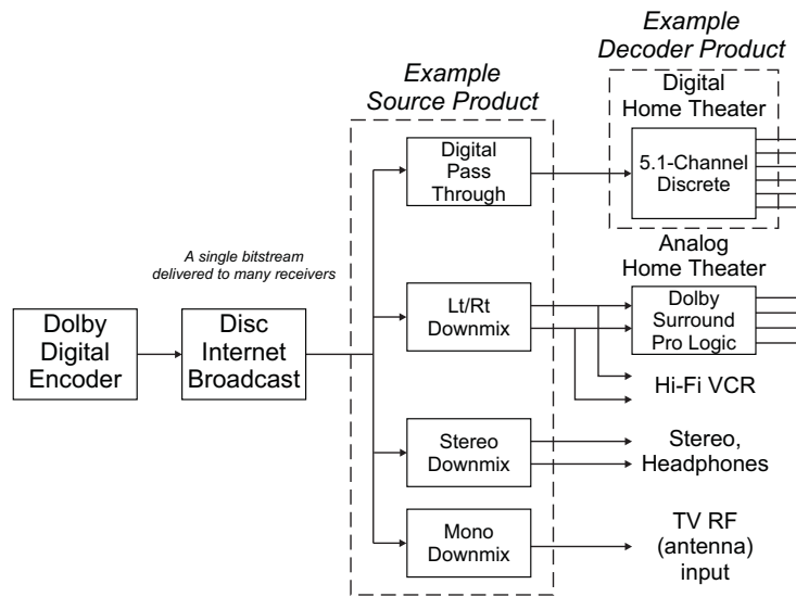
Figure 3-1 Audio Reproduction Hierarchy
