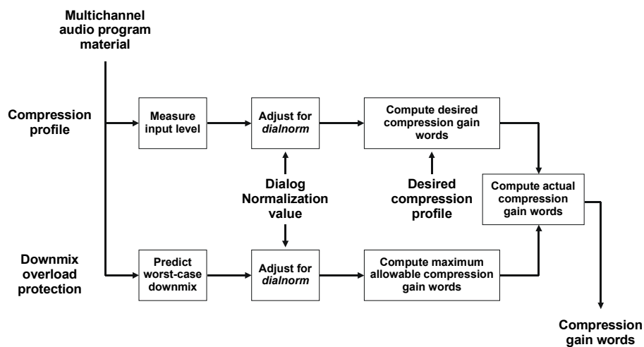
Figure C-1 Overview of Dynamic Range Control Algorithm
