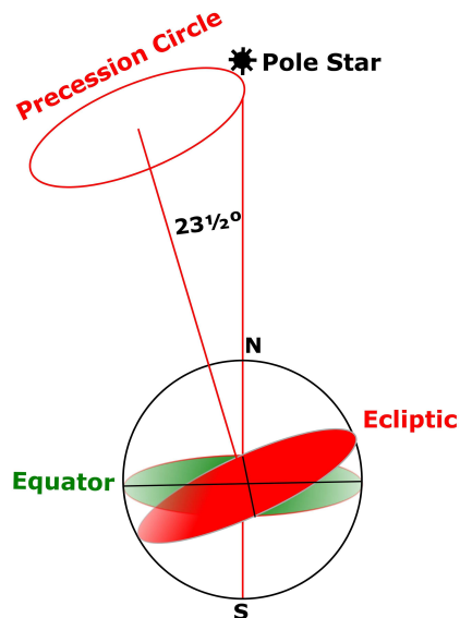
Precession of the Earth's polar axis
