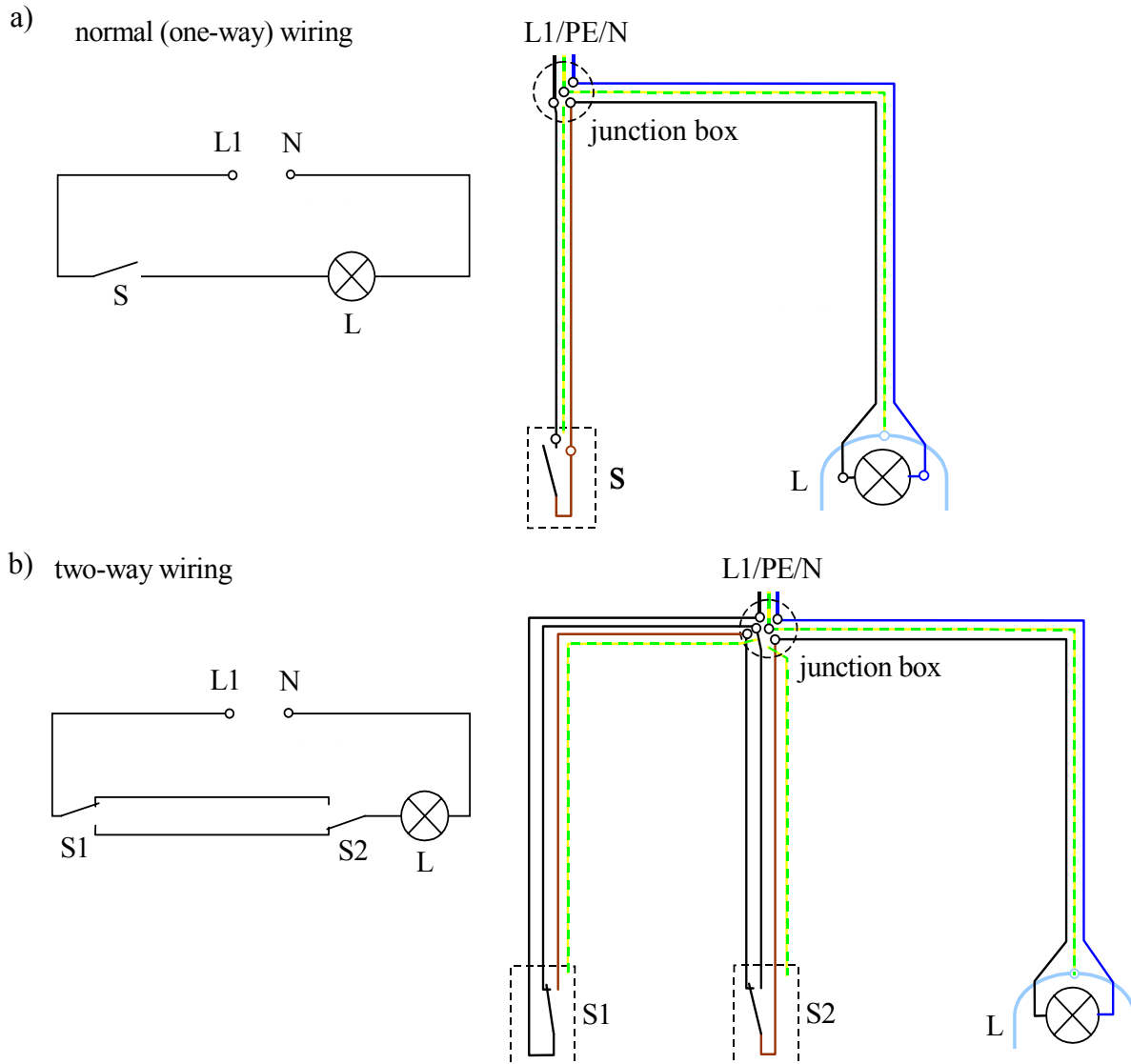
Figure 3.1.4-3: Lamp Circuits with One- and Two-Way Wiring.
