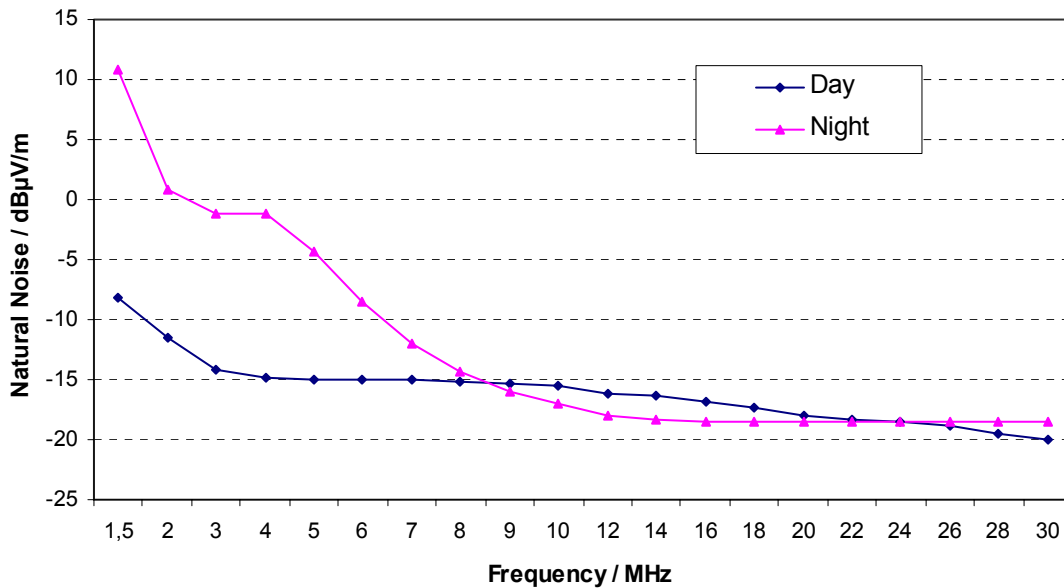
Figure 2.3-3: Low Natural Noise Measured in Germany.
