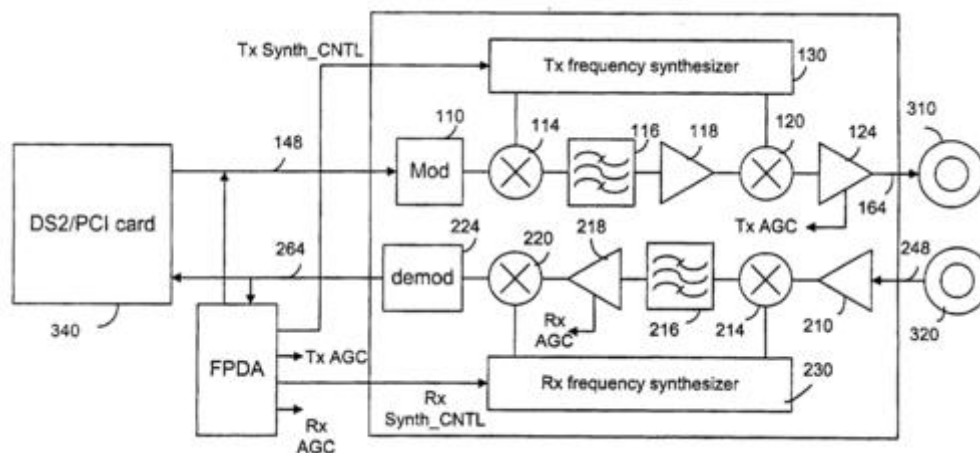
Figure 3.1.8-3: Amperion Injector/Extractor.
