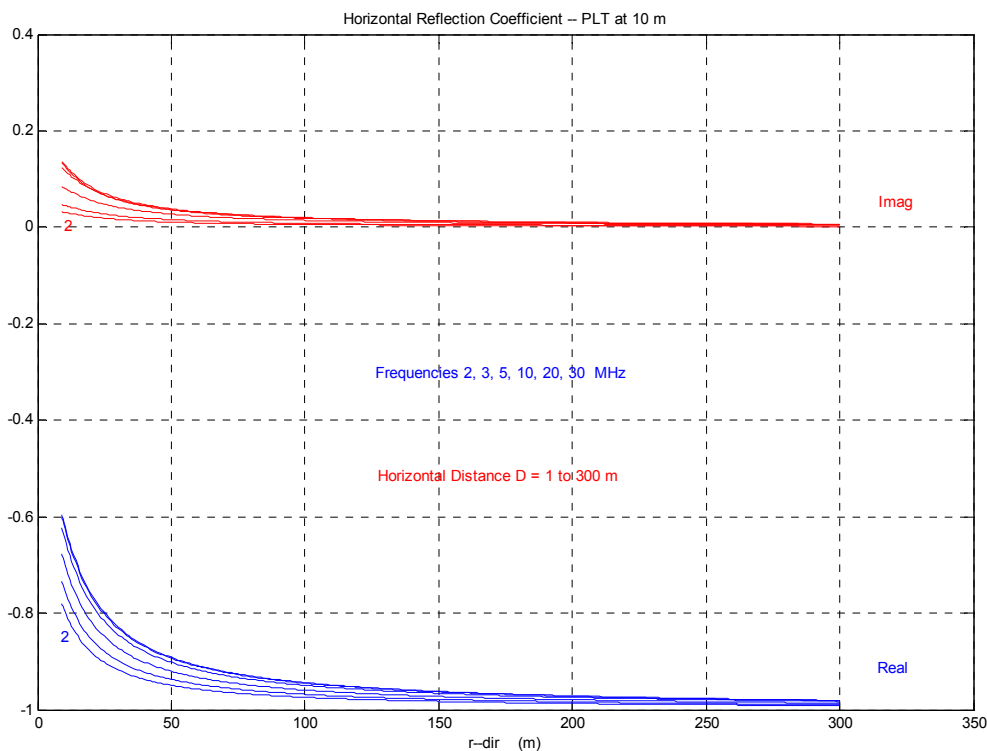
Figure 7.4.2.1-1: Horizontal Reflection Coefficient Profile – PLT Line Height at 10 Metres.
