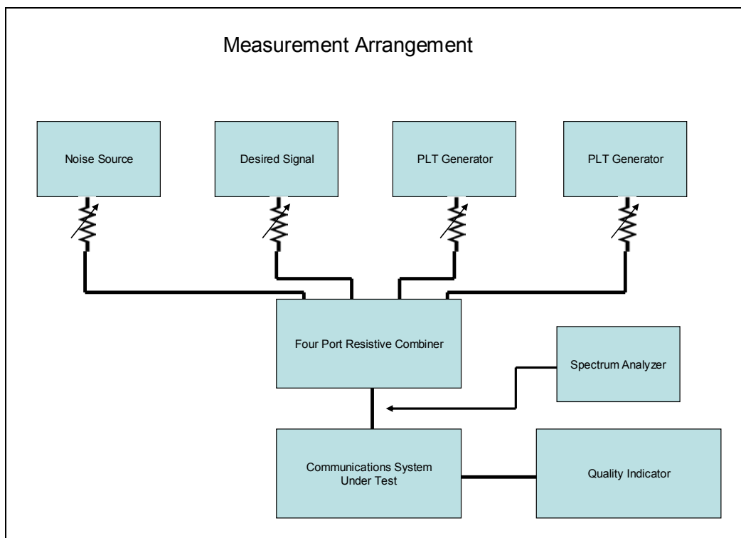
Figure 5.5-1: Measurement Arrangement.
