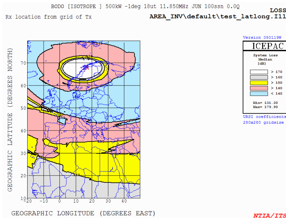
Figure 6.2-3: Example ICEPAC Output with Input Parameters as Recommended by the Task Group, using a Lat/Long Grid. Note that the results are identical to Figure 6.2-2 except from the representation (grid, projection and colour coding is different).
