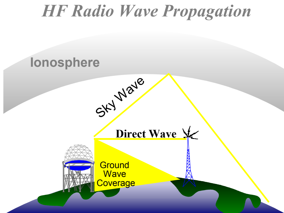
Figure 2.1-1: HF Radio Wave Propagation.
