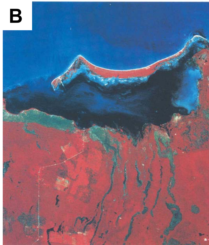
Figure 48. Landsat images. A - Hamelin Basin, Shark Bay, Australia. The embayment plain in the center of Hamelin Basin slopes from about 6 m depth in the south to 9 m in the north. B - Yalahau Lagoon, Yucatan, Mexico. Both lagoons are characterized by bioturbated muddy carbonate sediment.
