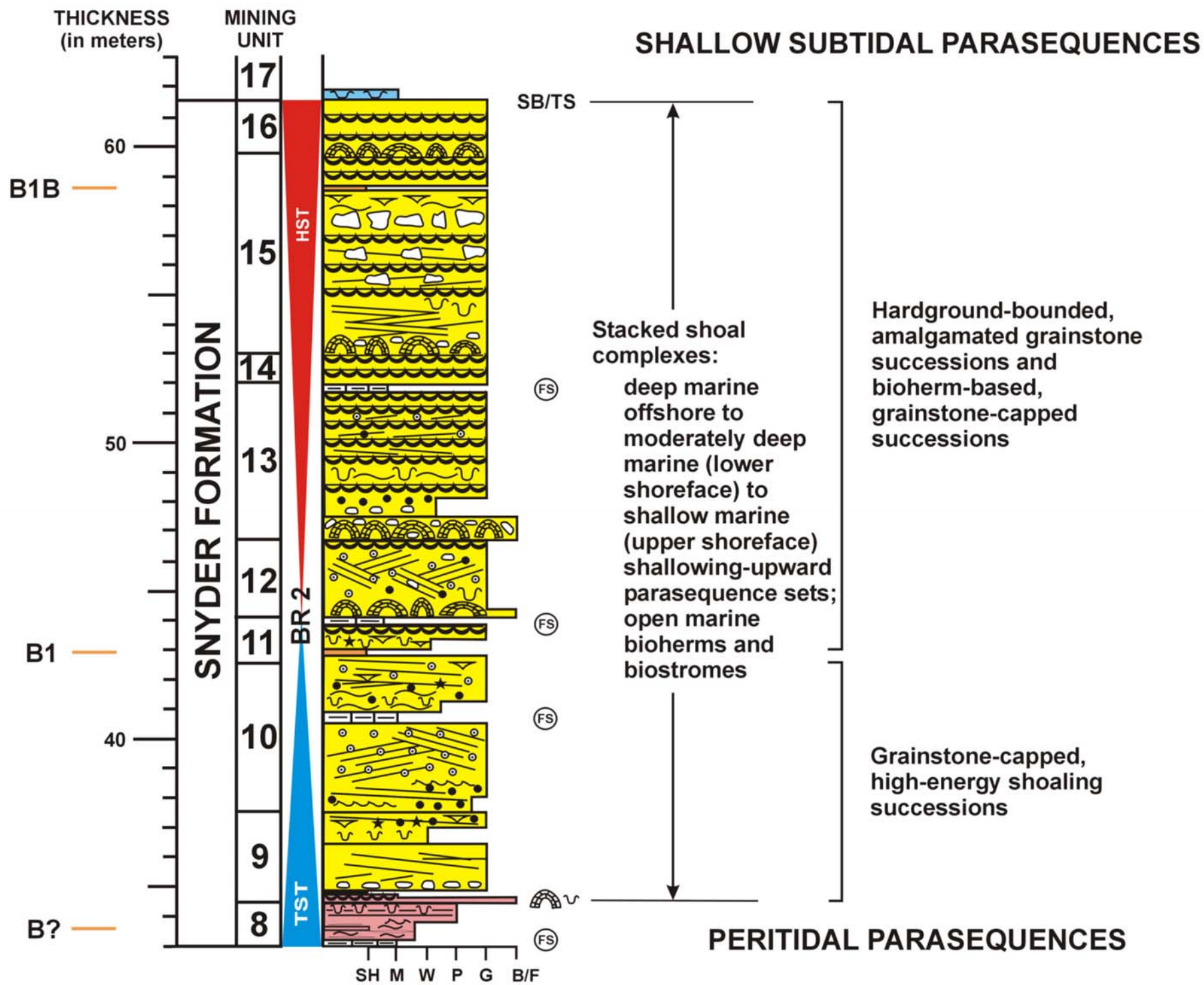
Figure 51. Vertical facies successions in the Snyder Formation exposed along Route 453 near Union Furnace, Pennsylvania. See Figure 18 for symbol legend. HST-highstand systems tract; TST-transgressive systems tract; SB/TS-combined sequence boundary/transgressive surface; FS-flooding surface.
