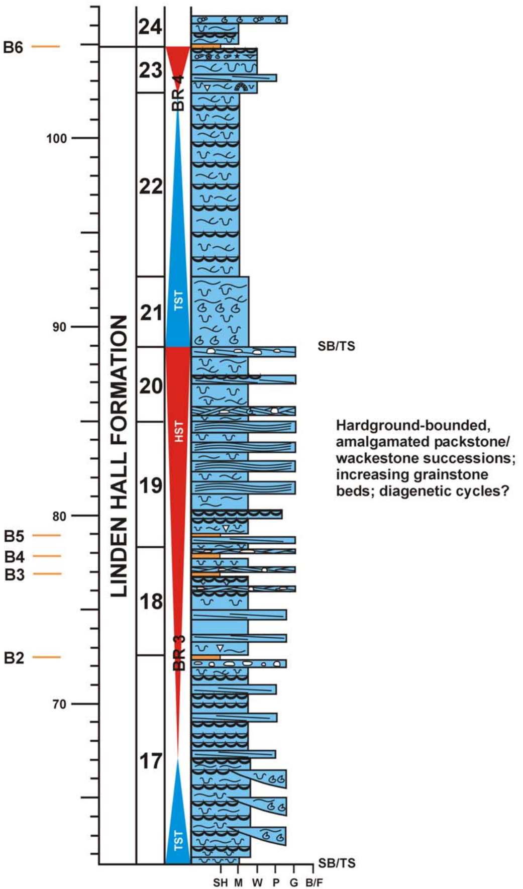
Figure 56. Vertical succession of sedimentary features in the Linden Hall Formation at Union Furnace. See Figure 18 for symbol legend. HST-highstand systems tract; TST-transgressive systems tract; SB/TS-combined sequence boundary/transgressive surface; FS-flooding surface.
