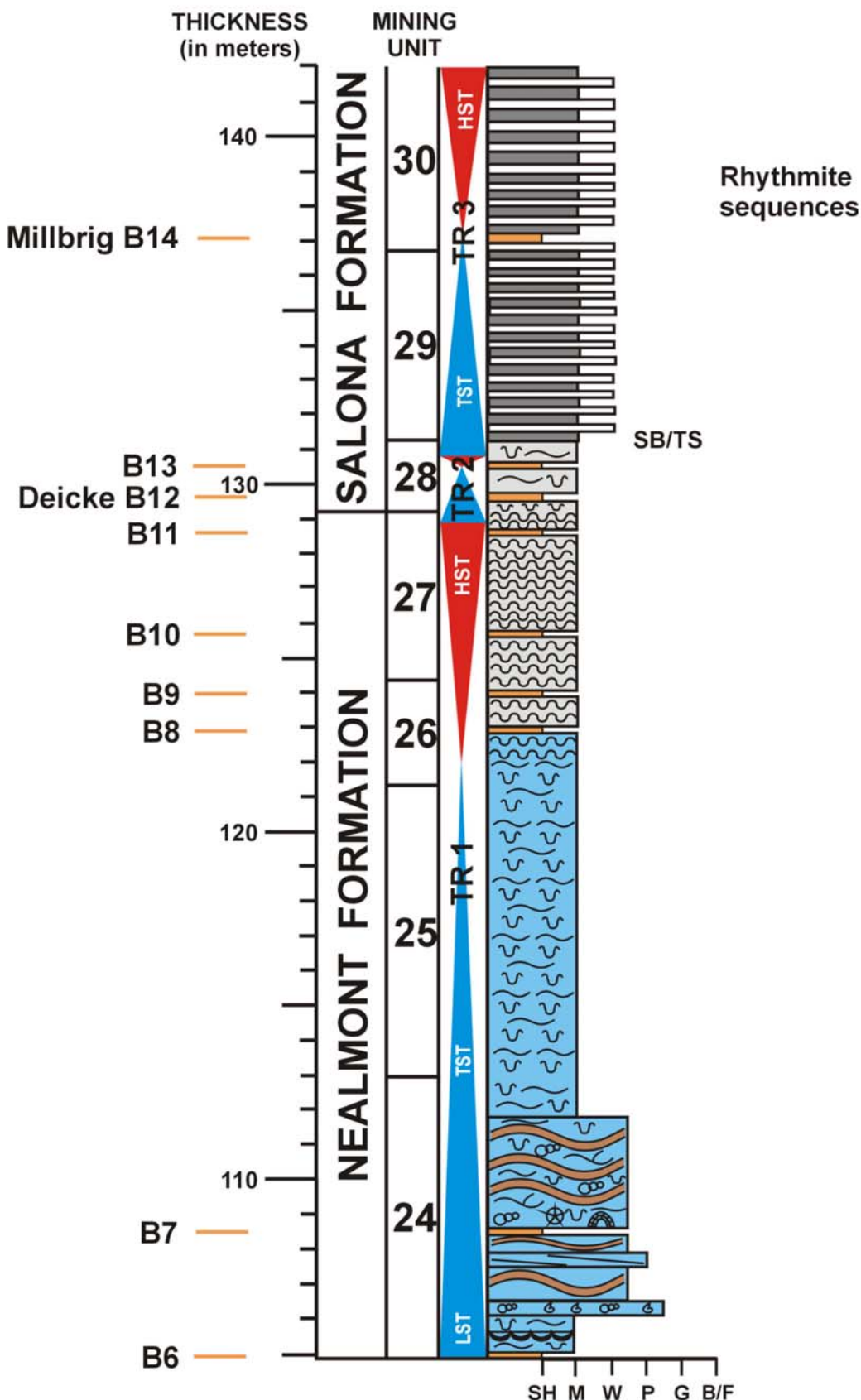
Figure 59. Vertical succession of sedimentary features in the Nealmont Formation and lowermost Salona Formation at Union Furnace. See Figure 18 for symbol legend. HST-highstand systems tract; LST-lowstand systems tract; TST-transgressive systems tract; SB/TS-combined sequence boundary/transgressive surface; FS-flooding surface.
