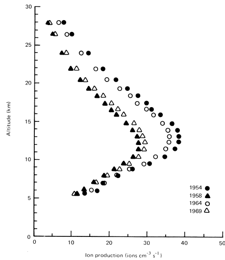
Figure 3. Variability over a solar cycle in the vertical profiles of Ion pair production over Thule, which is situated at a high magnetic latitude (adapted from Neher 1971). Due to geomagnetic shielding, the levels of ionisation are reduced at lower latitudes, but essential features in the vertical profile are similar.
