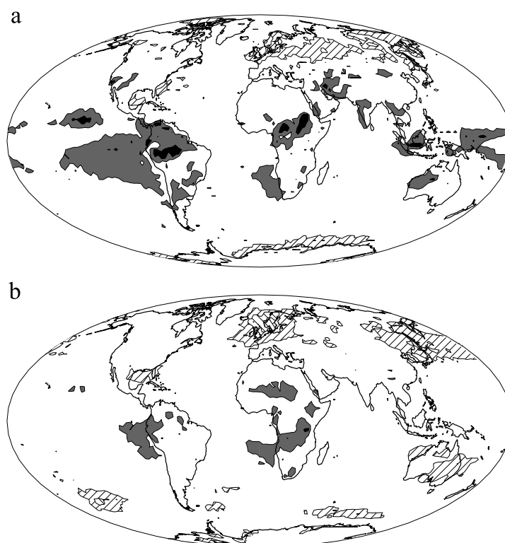
Figure 7. Global correlation maps of GCR with anomalies of a) atmospheric water vapour (1000-680hPa), and b) atmospheric temperature at 740 hPa. The water vapour and temperature are given by TOVS observations covering the period July 1983 - September 1994 (Rossow, 1996). Anomalies and correlation coefficients are calculated as in figure 5 and 6 (see both figure captions). The shading corresponds to filled contours, where correlation coefficient r > 0.8 - black, r > 0.6 - grey, and r < -0.6 - hatched, there are no regions with r < -0.8 . The fraction of Earth possessing a correlation coefficient > 0.6 is a) 11.7 % and b) 3.4 % which is not significant.
