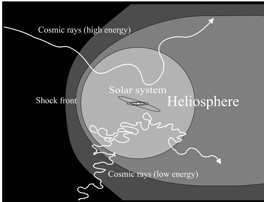
Figure 1. Schematic of Heliosphere
