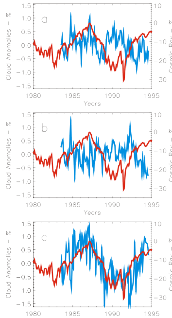
Figure 5. Monthly mean values for global anomalies of; a) high (<440hPa), b) middle (440 - 680hPa), and c) low (>680hPa) cloud cover (blue). Galactic cosmic ray fluxes (GCR) from Climax (red, normalised to May 1965) are used as a proxy for solar variability. The global average of the temporal mean over this period for high, middle and low IR detected clouds is 13.5 %, 19.9 %, and 28.0 % respectively.
