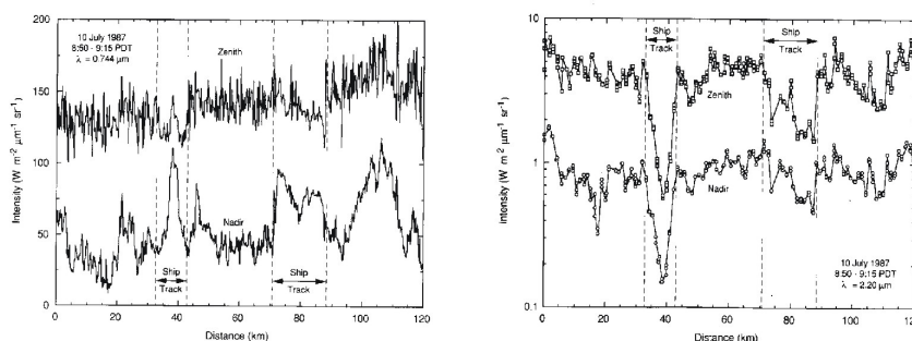
Figure 10. Visible 0.7 \mu\text{m} (left) and Near IR 2.2 \mu\text{m} (right) aircraft observations of ship tracks in low cloud (adapted from King et al, 1993).
