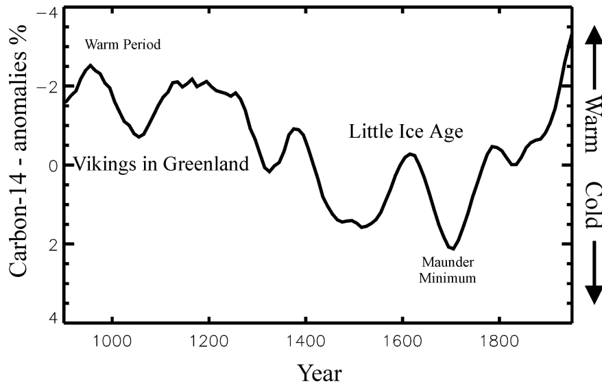
Figure 12. Changes in ^{14}\text{C} levels over the past 1000 years relative to 1950. ^{14}\text{C} is produced through nuclear interactions of cosmic ray particles in the atmosphere. Cosmic rays are modulated by the solar wind; thus, variability in ^{14}\text{C} production is mainly a result of changes in solar activity. High solar activity leads to stronger shielding from the solar wind and thus a reduction in the production rate. Note the inverted axis for ^{14}\text{C} anomalies. The sharp deviation of ^{14}\text{C} during the last century is due to the burning of ^{14}\text{C} depleted fossil fuels (the Suess effect).
