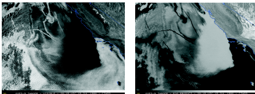
Figure 9. Images of Ship Condensation Trails Off the California Coast taken on 15 July 1998 by GOES-9. Left image is in the Visible ( 0.7 \mu\text{m} ) and right image is the IR Fog Product ( 10.7 \mu\text{m} - 3.9 \mu\text{m} ).
