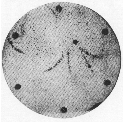
Figure 3: A group of six particles projected from a region in the wall of the chamber. The track at the left of the central group of four tracks is a negatron of about 18 million volts energy ( H\rho = 6.2 \times 10^4 gauss-cm) and that at the right a positron of about 20 million volts energy ( H\rho = 7.0 \times 10^4 gauss-cm). Identification of the two tracks in the center is not possible. A negatron of about 15 million volts is shown at the left. This group represents early tracks which were broadened by the diffusion of the ions. The uniformity of this broadening for all the tracks shows that the particles entered the chamber at the same time.
