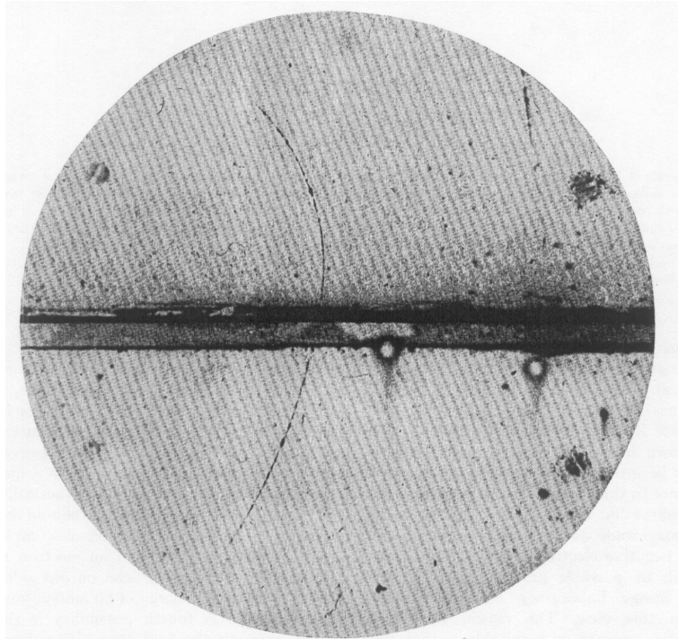
Figure 1: A 63 million volt positron ( H\rho = 2.1 \times 10^5 gauss-cm) passing through a 6 mm lead plate and emerging as a 23 million volt positron ( H\rho = 7.5 \times 10^4 gauss-cm). The length of this latter path is at least ten times greater than the possible length of a proton path of this curvature.
