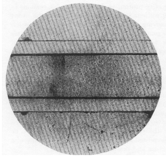
Figure 2: A positron of 20 million volts energy ( H\rho = 7.1 \times 10^4 gauss-cm) and a negatron of 30 million volts energy ( H\rho = 10.2 \times 10^4 gauss-cm) projected from a plate of lead. The range of the positive particle precludes the possibility of ascribing it to a proton of the observed curvature.
