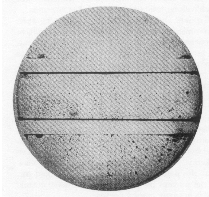
Figure 4: A positron of about 200 million volts energy ( H\rho = 6.6 \times 10^5 gauss-cm) penetrates the 11 mm lead plate and emerges with about 125 million volts energy ( H\rho = 4.2 \times 10^5 gauss-cm). The assumption that the tracks represent a proton traversing the lead plate is inconsistent with the observed curvatures. The energies would then be, respectively, about 20 million and 8 million volts above and below the lead, energies too low to permit the proton to have a range sufficient to penetrate a plate of lead of 11 mm thickness.
