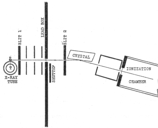
Figure 1: Measuring the wave-length of scattered X -rays.
