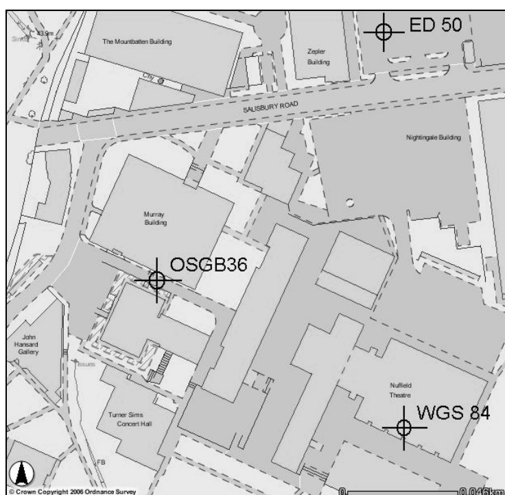
Figure 1: Three points with the same latitude and longitude in three different coordinate systems. The map extract is 200 metres square.
