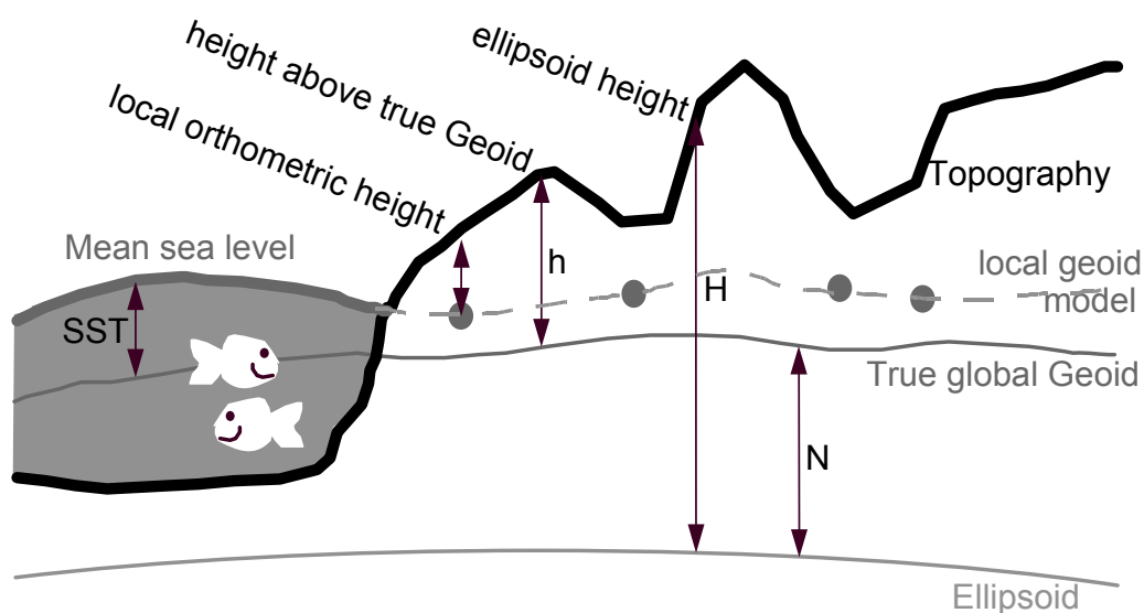
Figure 7: The relationship between the Geoid, a local geoid model (based on a tide-gauge datum), mean sea level, and a reference ellipsoid. The ODN geoid model is an example of a local geoid model.
