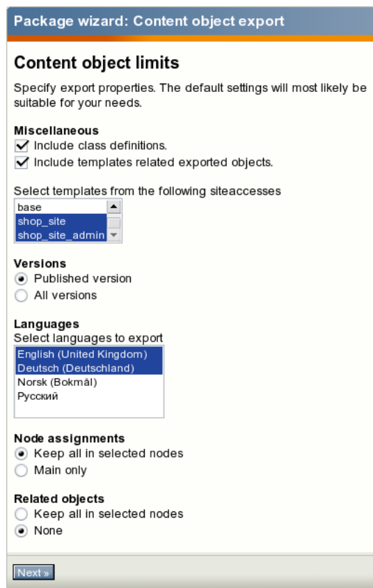
Figure 4.36: The content object package creation wizard: export properties for content objects.
