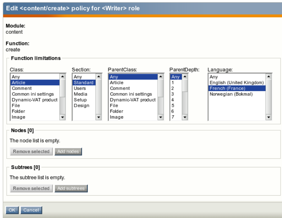
Figure 4.19: The policy edit interface.
