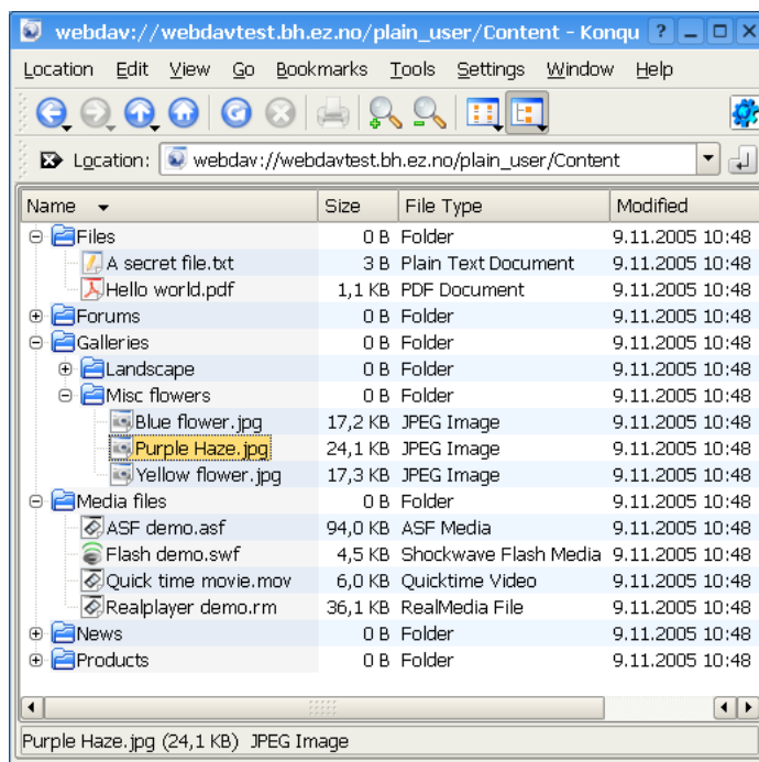
Figure 4.129: WebDAV - Content node tree
