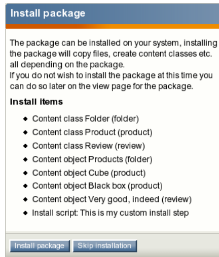
Figure 4.58: Displaying a custom install script in the list of items during the package installation process
