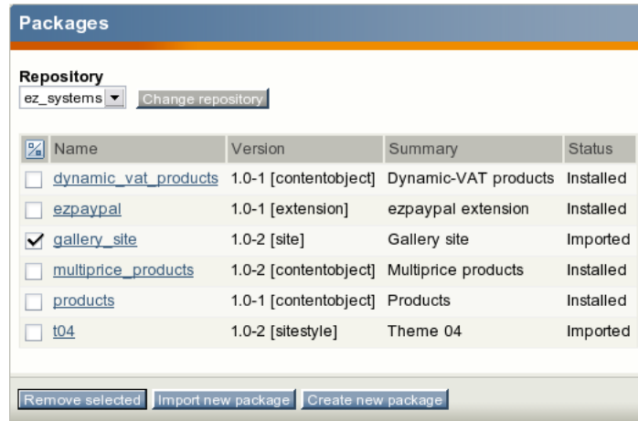
Figure 4.45: Removing a package.
