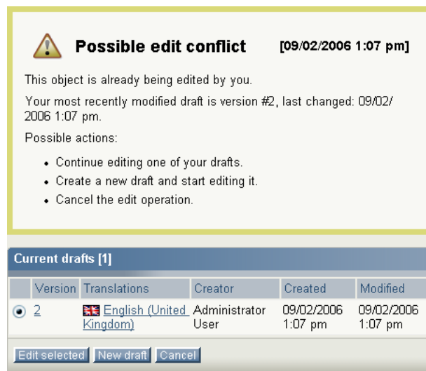
Figure 2.9: Edit conflict - same user.
