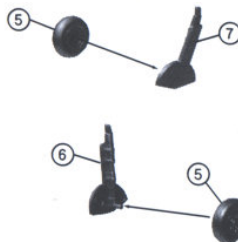
5 Assembly of the landing gear
