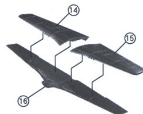
3 Assembly of wings
