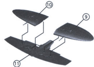
3 Assembly of wings
