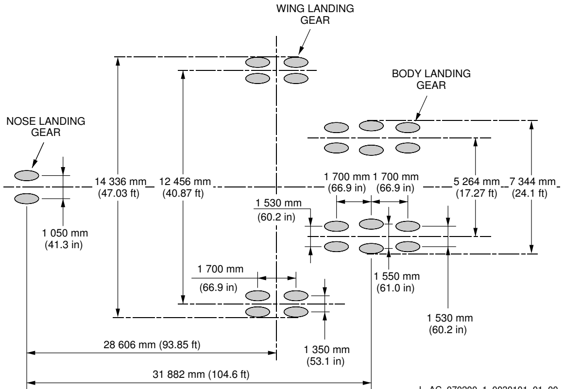
Landing Gear Footprint MRW 512 000 kg - A380-800 Models
