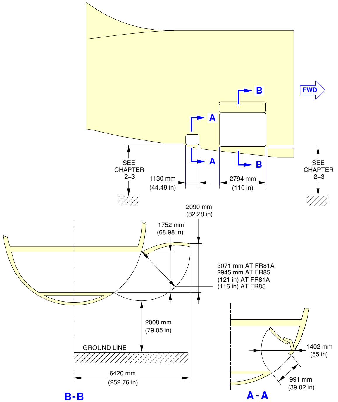
Door Clearances Lower Deck Aft Cargo Doors - A380-800F Models
