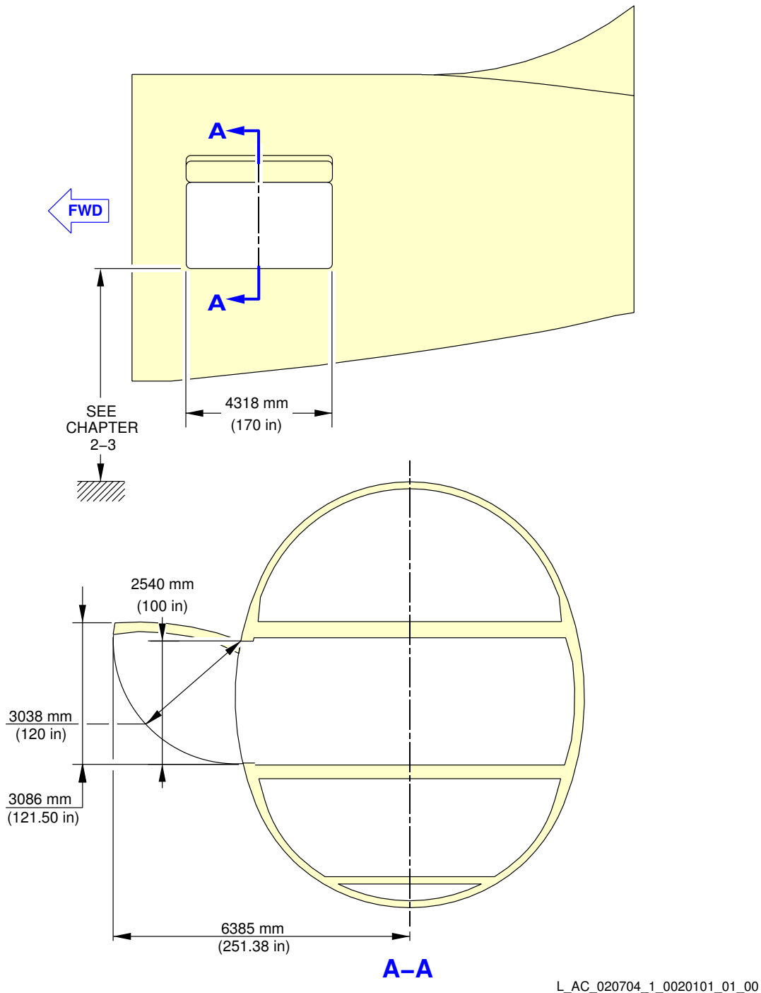
Door Clearances Main Deck Cargo Door - A380-800F Models
