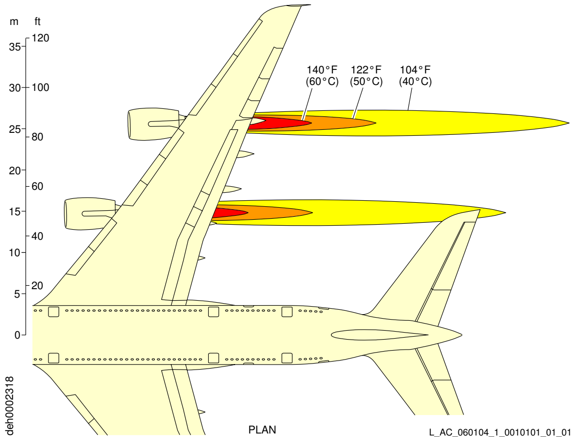
Engine Exhaust Temperatures Breakaway Power - TRENT 900 Engines
