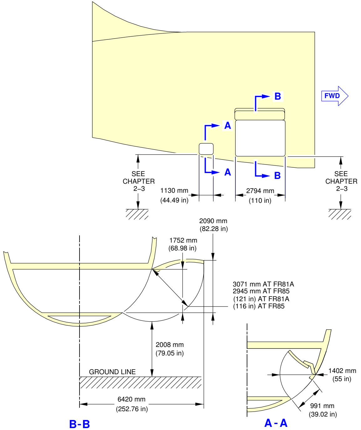
Door Clearances Aft Cargo Compartment Doors - A380-800 Models
