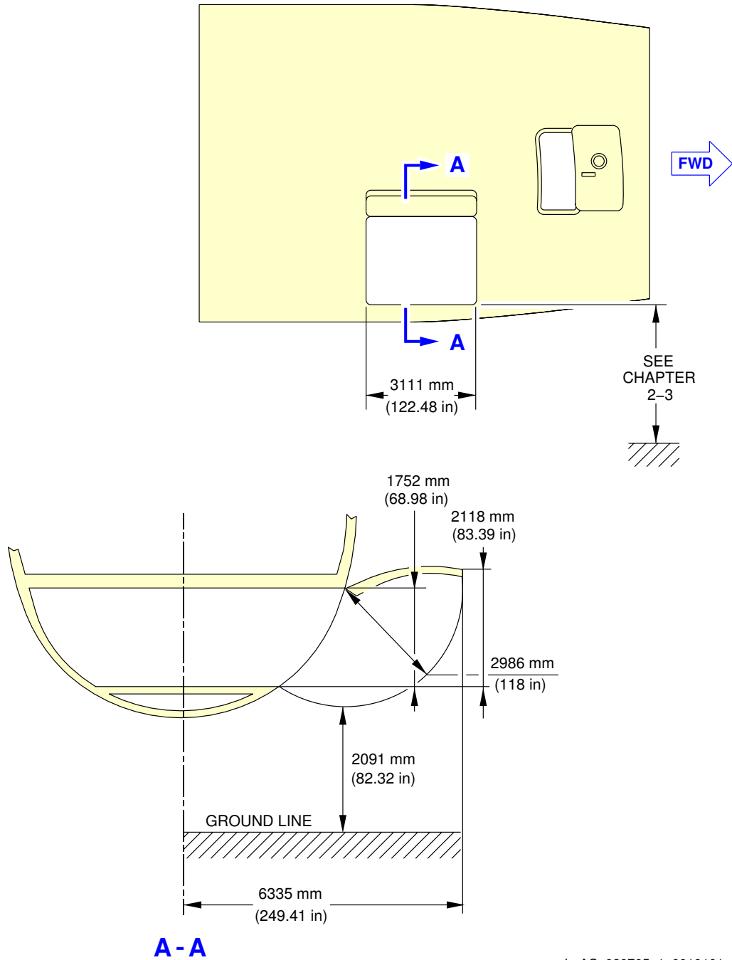
Door Clearances Forward Cargo Compartment Doors - A380-800 Models
