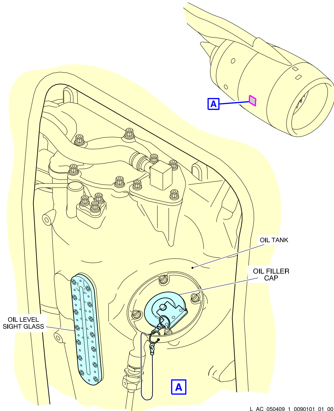
Ground Service Connections Engine Oil Servicing - TRENT 900 Engines
