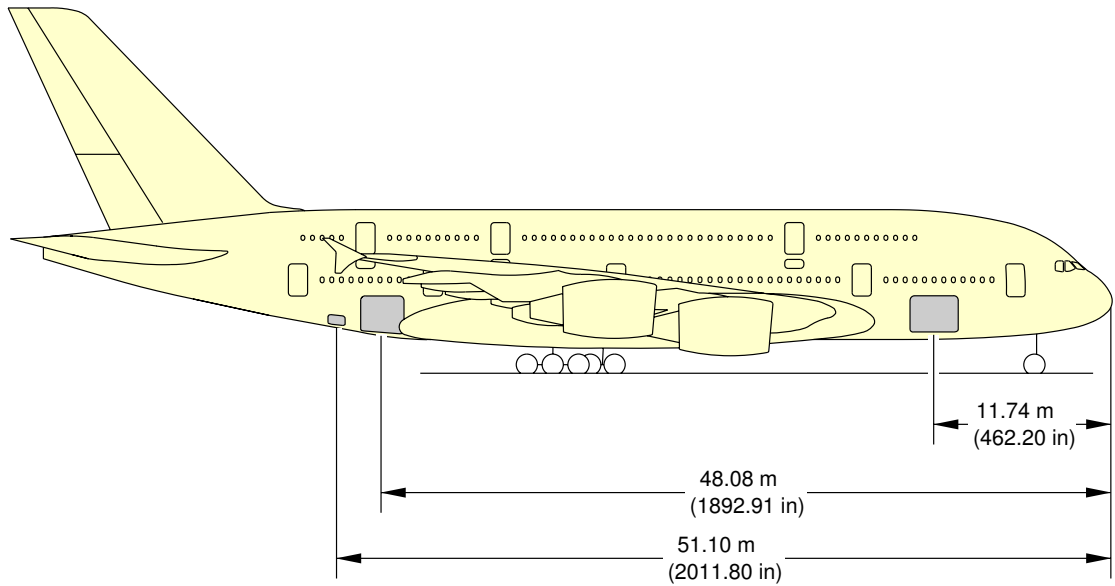
Door Clearances Door Location (Sheet 2) - A380-800 Models
