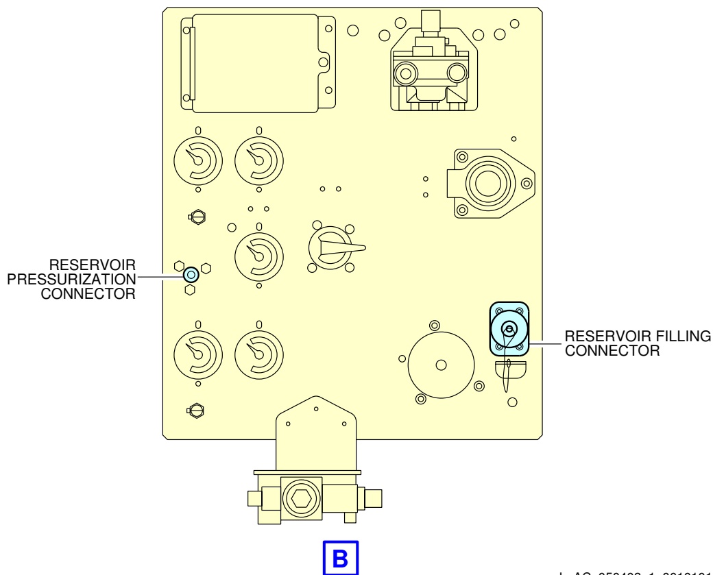
Ground Service Connections Hydraulic Reservoir Servicing Panel
