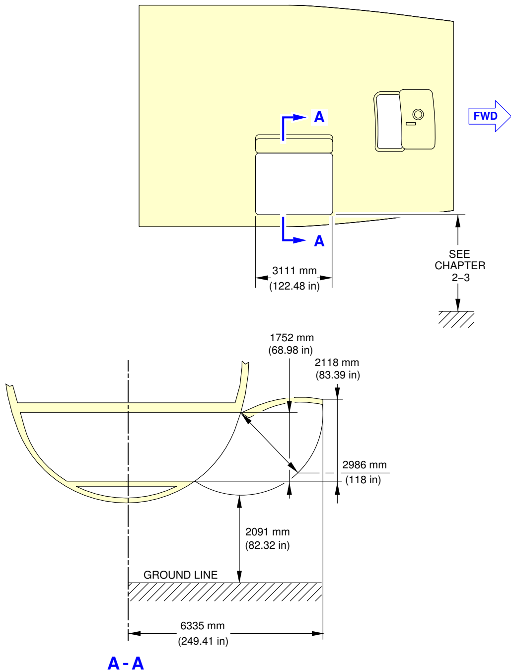
Door Clearances Lower Deck Forward Cargo Door - A380-800F Models
