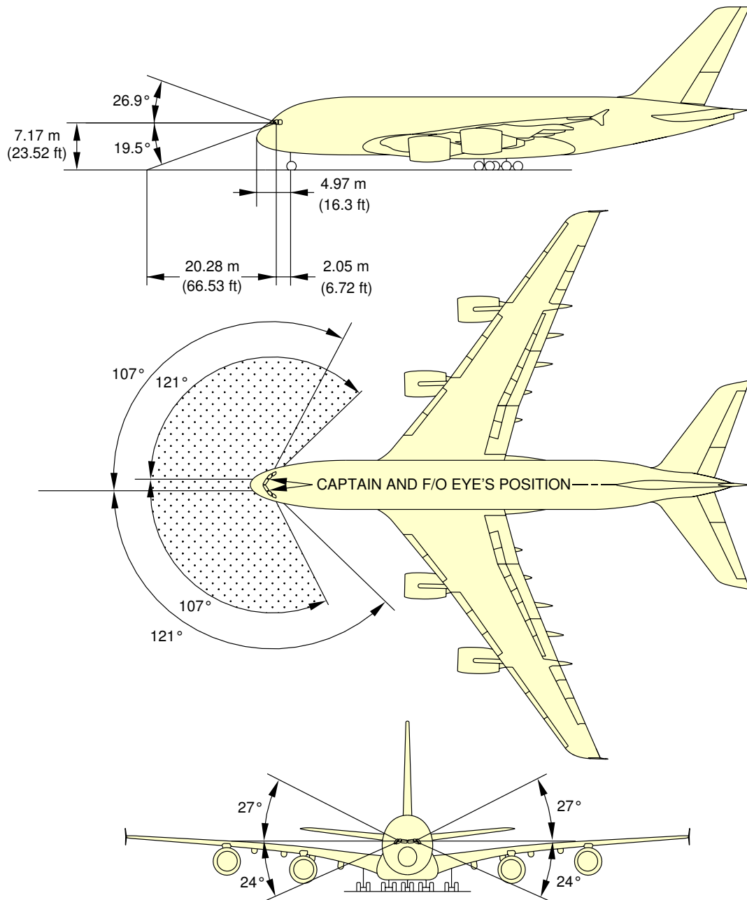
Visibility from Cockpit in Static Position
