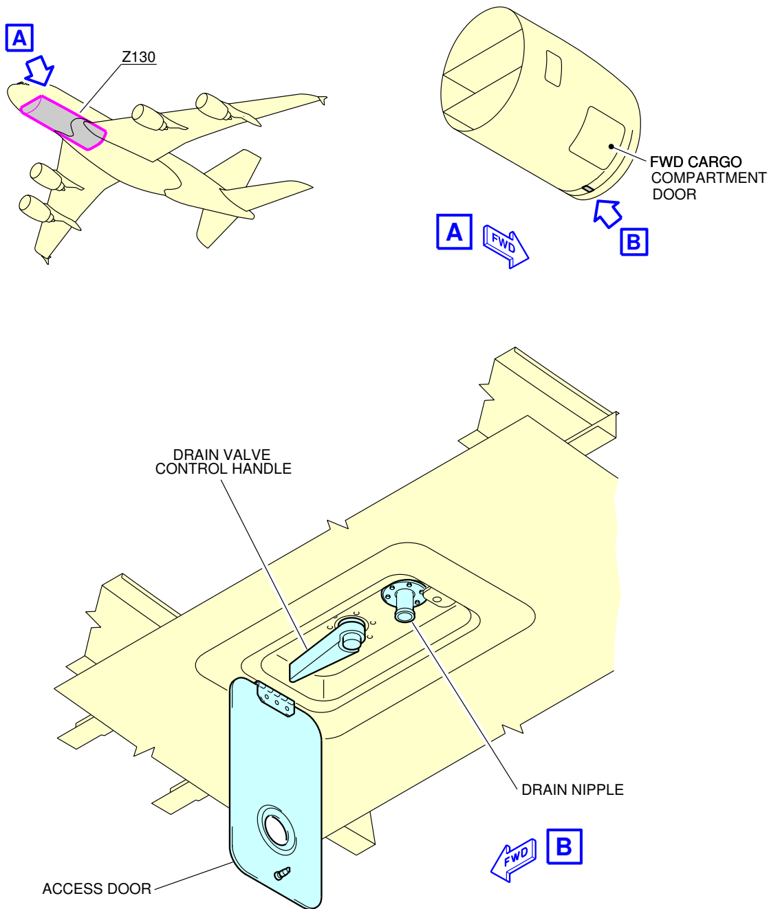
Ground Service Connections Potable Water Drain Panel - A380-800 Models
