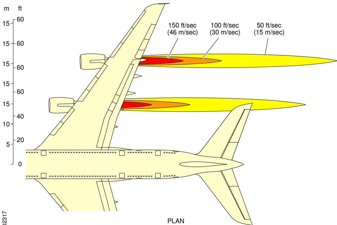
Engine Exhaust Velocities Ground Idle Power - TRENT 900 Engines
