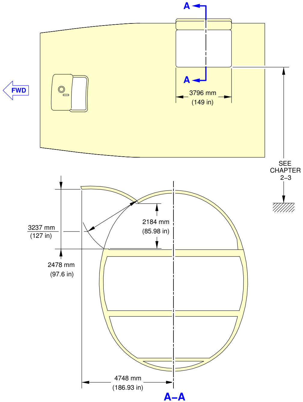
Door Clearances Upper Deck Cargo Door - A380-800F Models
