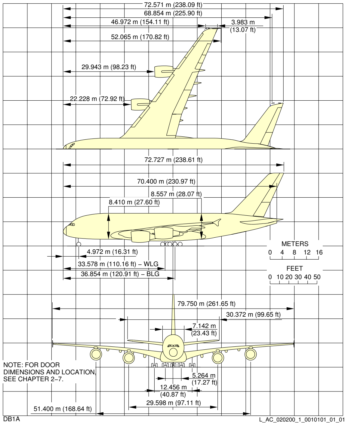
General Airplane Dimensions
