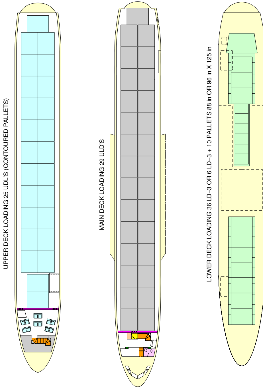
Cargo Compartments Loading Combinations (Sheet 1)
