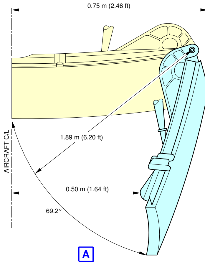
Door Clearances Aft Nose Landing Gear Doors
