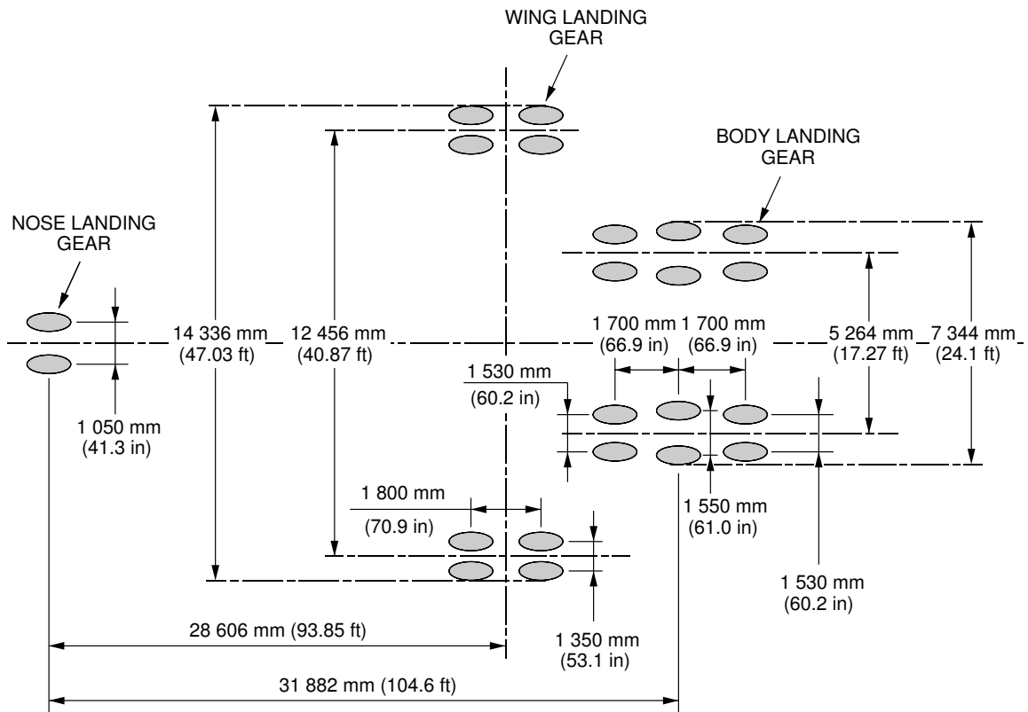
Landing Gear Footprint MRW 602 000 kg - A380-800F Models
