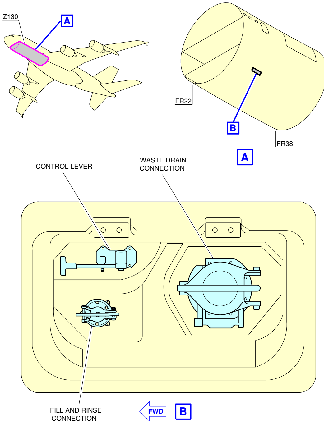
Ground Service Connections Vacuum Toilet System - A380-800F Models
