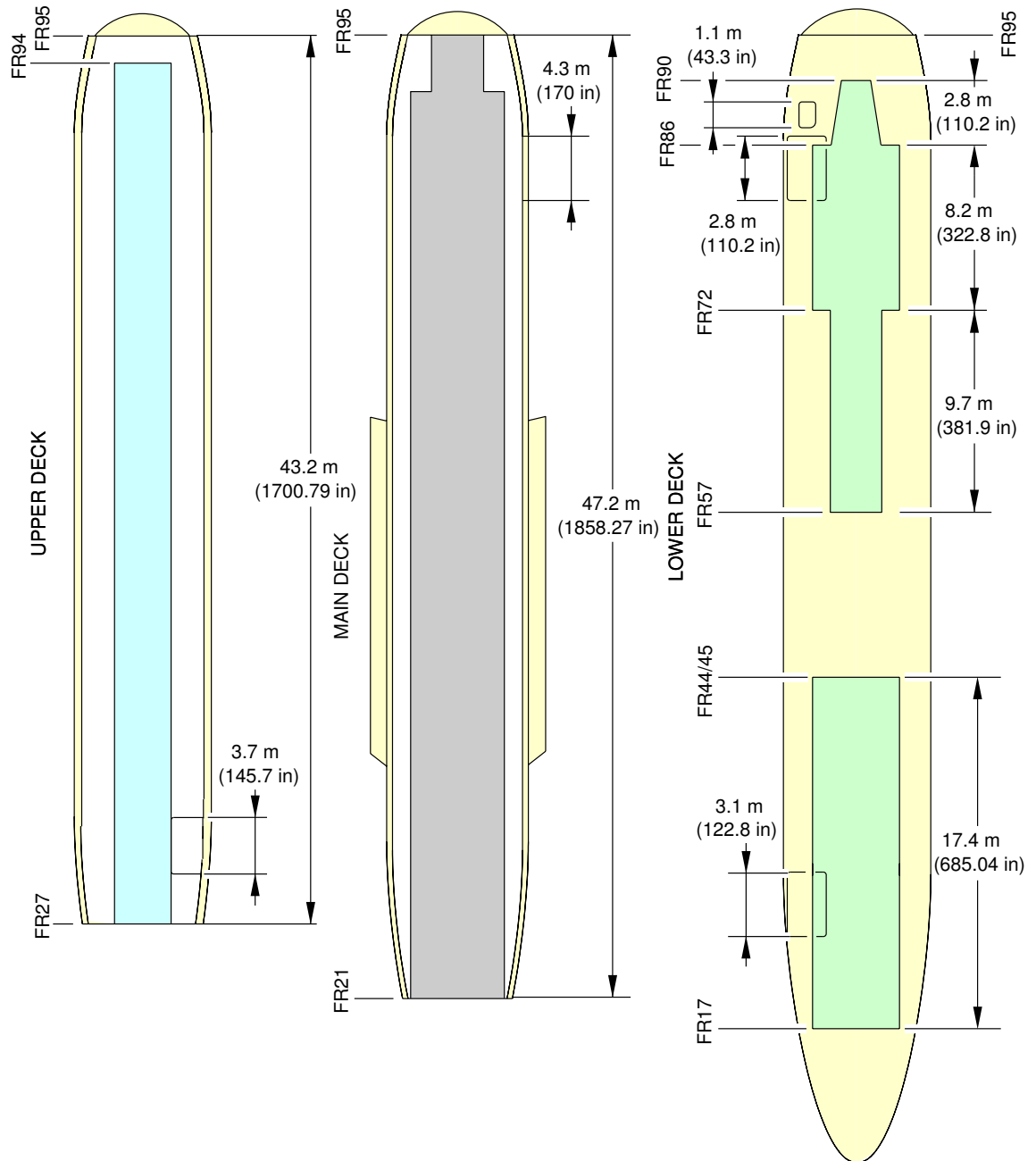
Cargo Compartments Location and Dimensions (Sheet 2)
