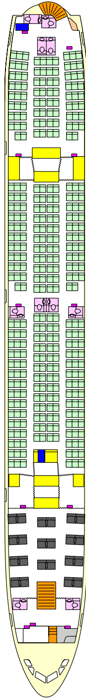
Interior Arrangements - Plan View Standard Configuration - Main Deck
