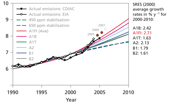
Observations of anthropogenic CO 2 emissions from 1990 to 2007. The envelope of IPCC projections are shown for comparison 12,18,34 . Coloured and stippled lines refer to different IPCC scenarios.
