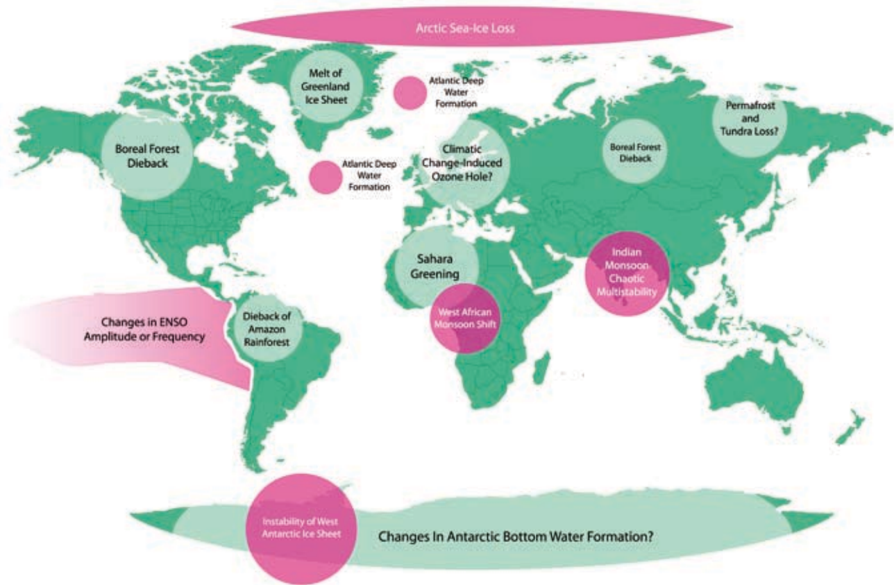
Figure 7 Map of potential climatic “tipping elements”. Tipping elements are regional-scale features of the climate that could exhibit threshold-type behaviour in response to human-driven climate change – that is, a small amount of climate change at a critical point could trigger an abrupt and/or irreversible shift in the tipping
