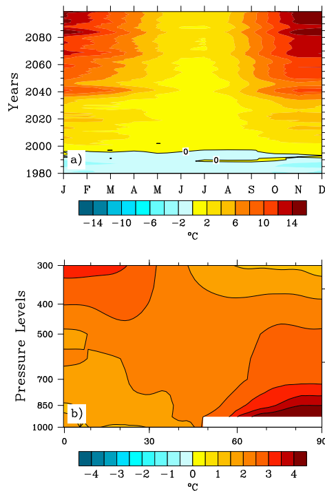
Fig. 1. NCAR CCSM3 depictions of: (a) near surface (2 m) temperature anomalies by month and year over the Arctic Ocean (see Fig. 3); and (b) latitude by height dependence of zonally-averaged October–March temperature anomalies for 2050–2059. Anomalies are relative to 1979–2007 means. See Fig. 3 for definition of the Arctic Ocean domain.
