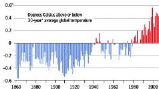
Figure 1. Derivation from global mean temperatures.
