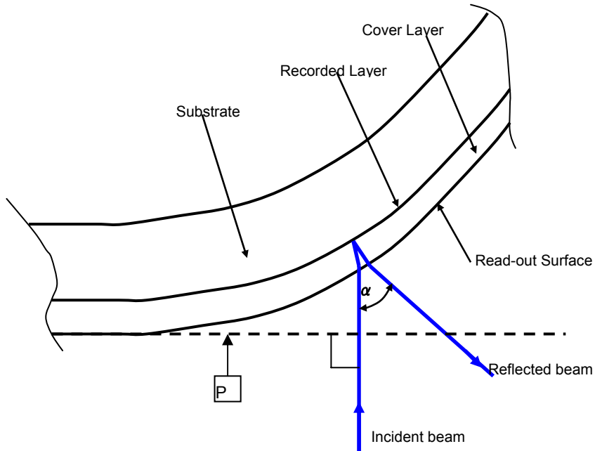
Fig.2-4 \alpha angle explanation
