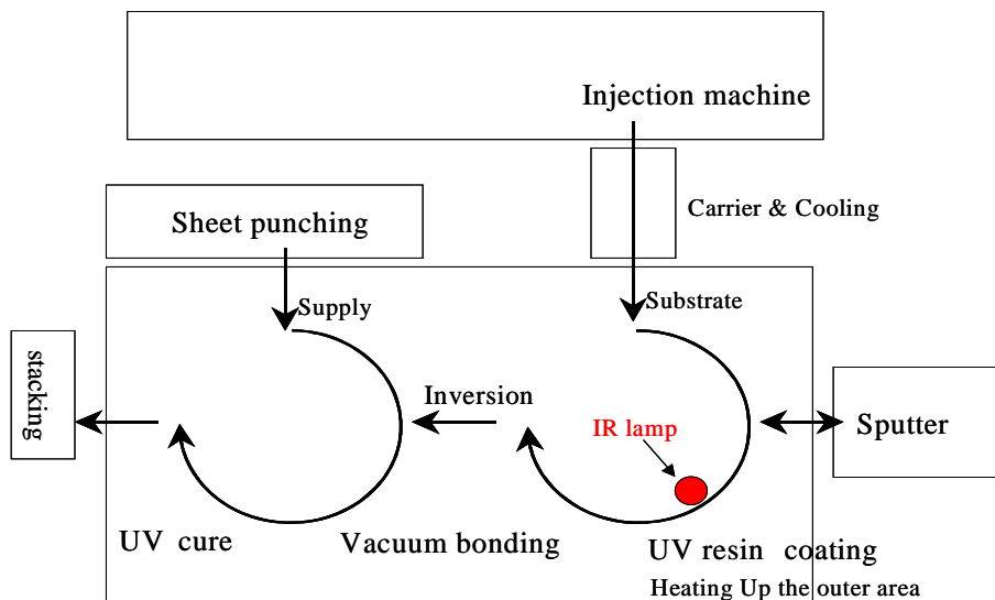
Fig.12-12 Single Layer process
