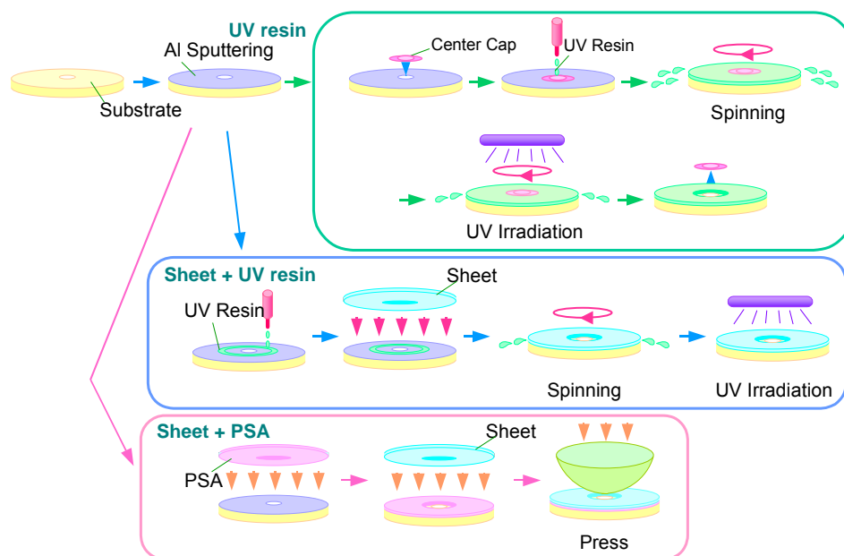
Fig.4-5 Cover Layer process
