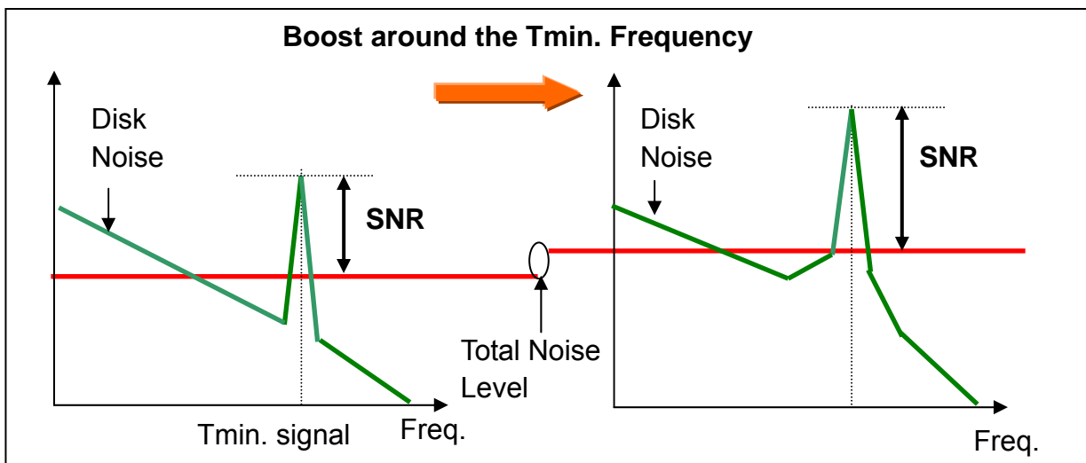
Fig.11-1 SNR improvement of a Limit-Equalizer
