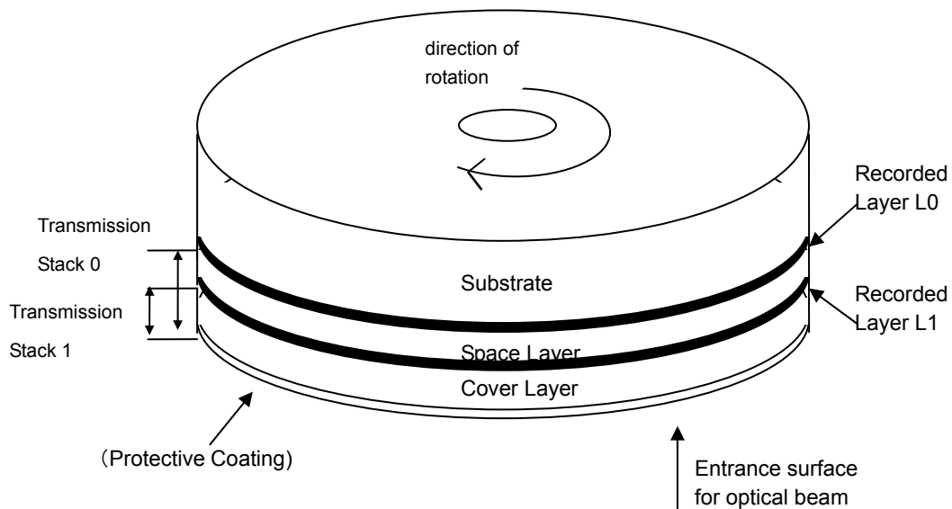
Fig.4-2 Outline of Dual Layer BD Read-Only disc
