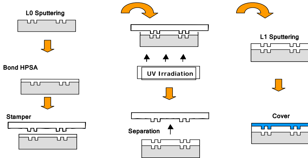
Fig.12-16 Manufacturing process for the Dual Layer disc
