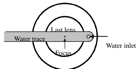
Fig.12-6 Liquid immersion concept
