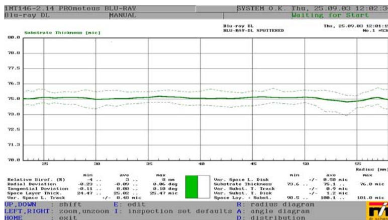
Fig.12-17 Thickness variation of L1 Layer
