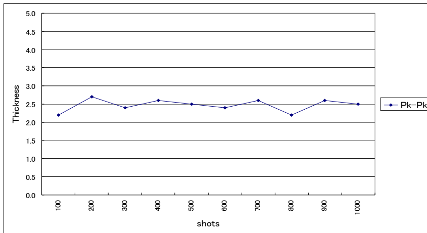
Fig.12-20 L0 thickness variation for a 1000 disc series
