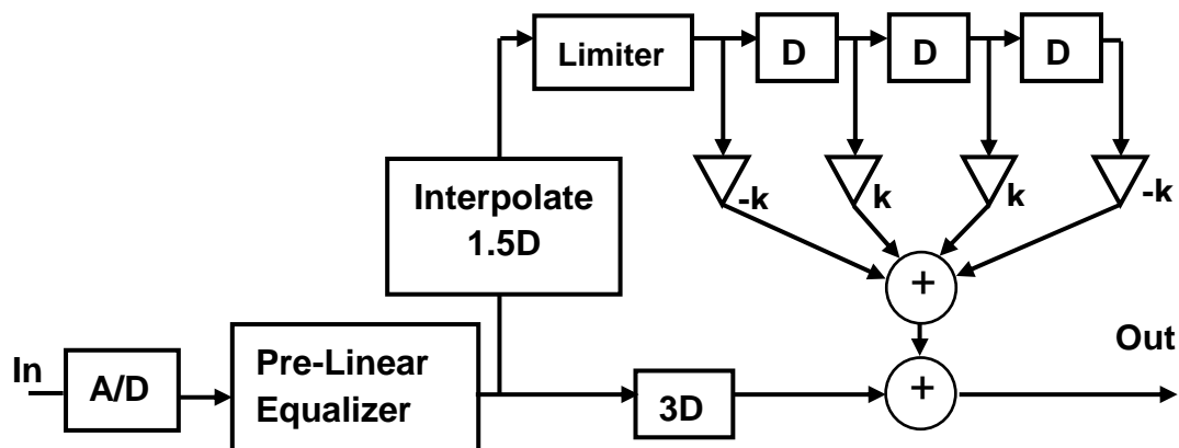
Fig.11-2 The configuration of a Limit-Equalizer
