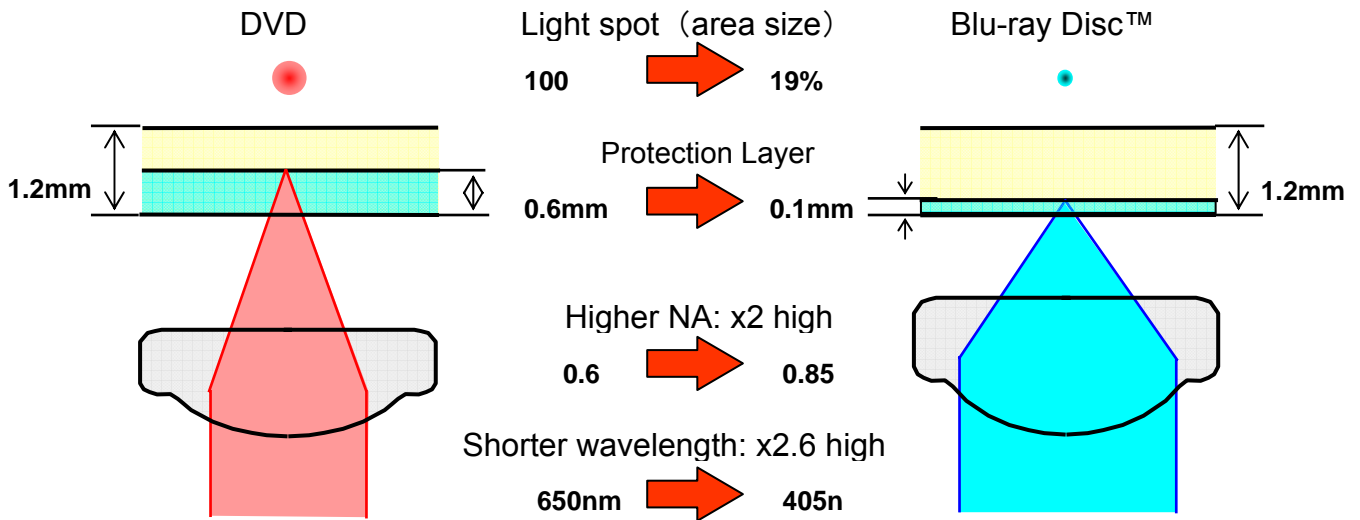
Fig.2-2 High-capacity contribution
