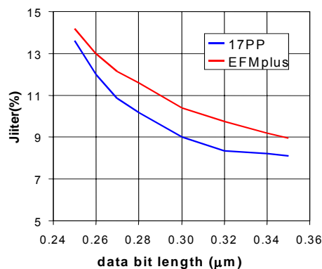
Fig.9-1 The density comparison in two modulation codes
