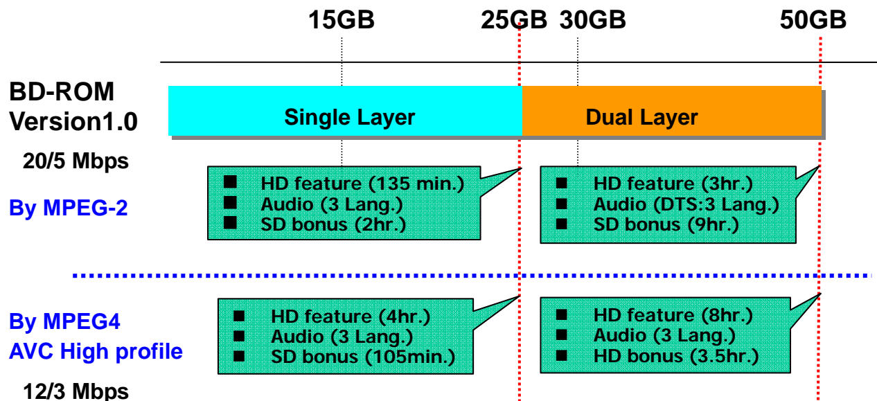
Fig. 2-1 BD-ROM version 1.0 capacity
