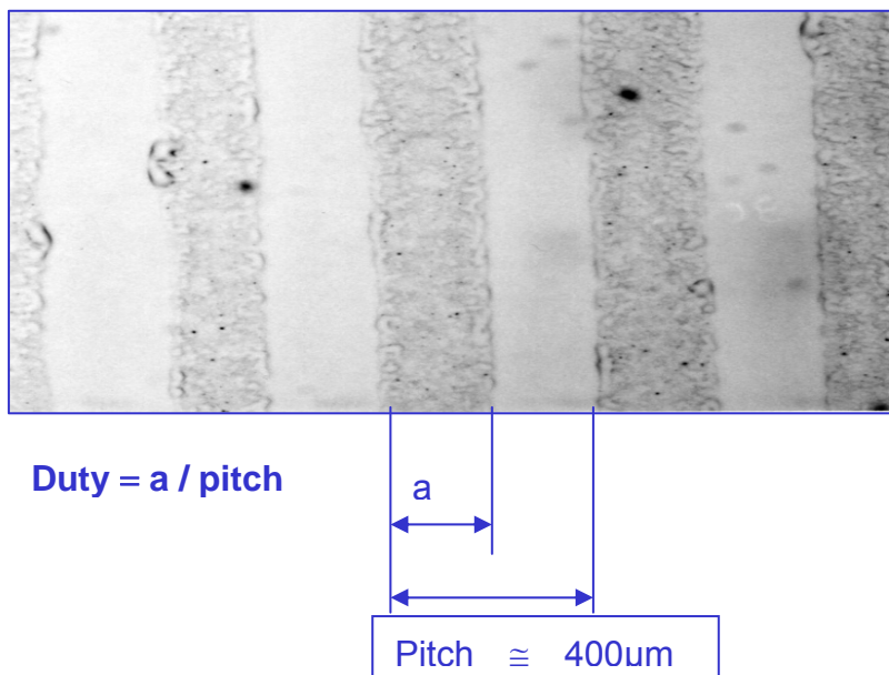
Fig.5-4 Artificial finger prints for the servo stability test
