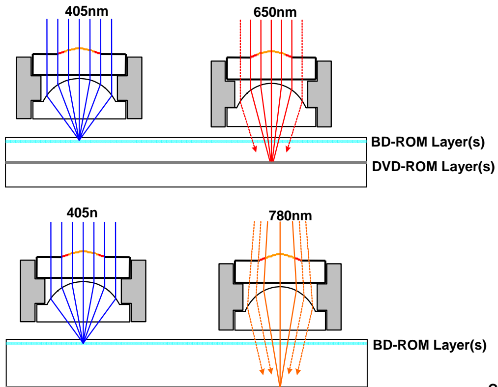
Fig. 16-1 Examples of ROM-ROM type Hybrid discs
