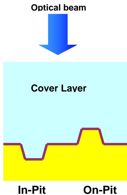
Fig. 7-1 Pit shape
