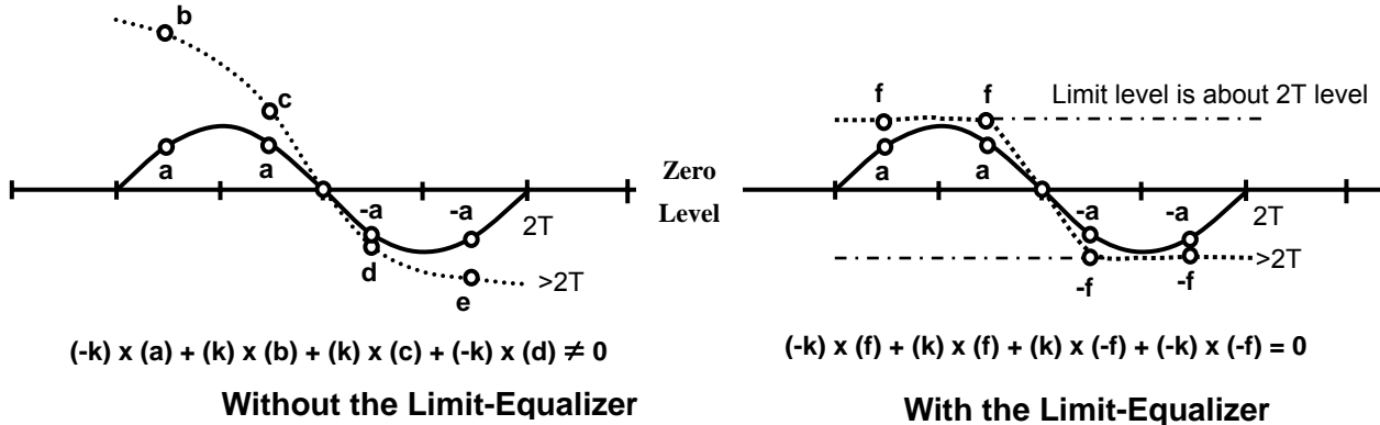
Fig.11-3 Behavior of a Linear Equalizer and Limit-Equalizer
