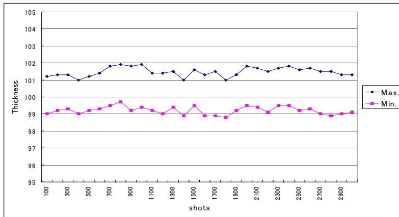
Fig.12-14 Cover thickness variation for a 3,000 disc series
