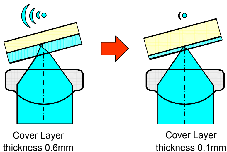
Fig.2-3 Necessity of 0.1 mm Cover Layer
