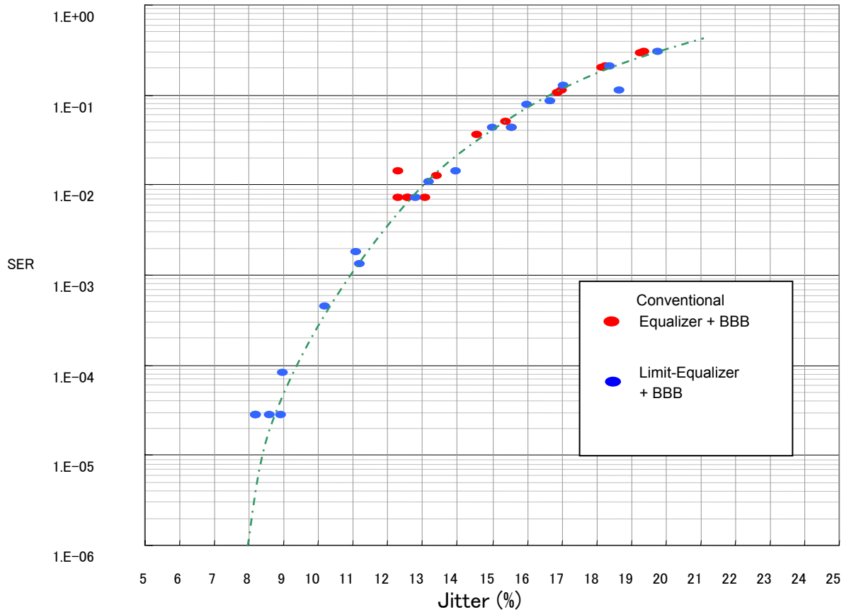
Fig.11-4 The relation of the error rate and Jitter of the Conventional Equalizer and the Limit-Equalizer
