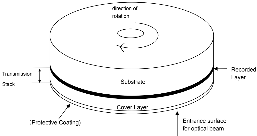
Fig.4-1 Outline of Single Layer BD Read-Only disc
