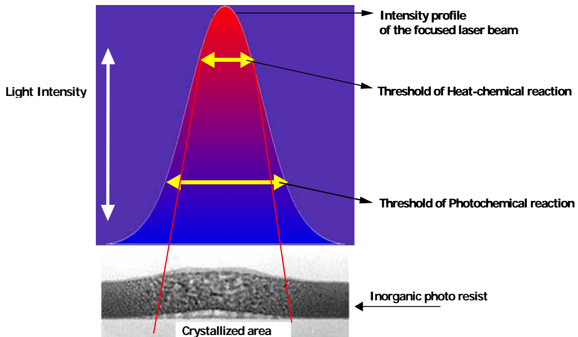
Fig.12-1 PTM recording mechanism
