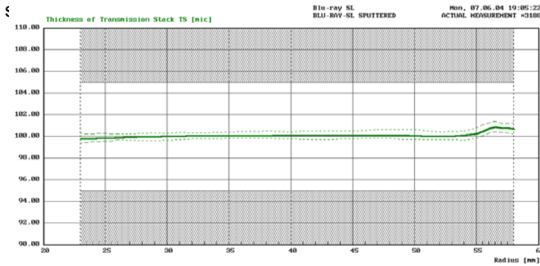
Fig.12-13 Thickness variation
