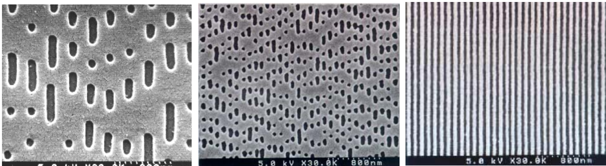
Fig.12-11 (a) 25GB ROM (b) 201 GB ROM (c) 50 nm line and space
