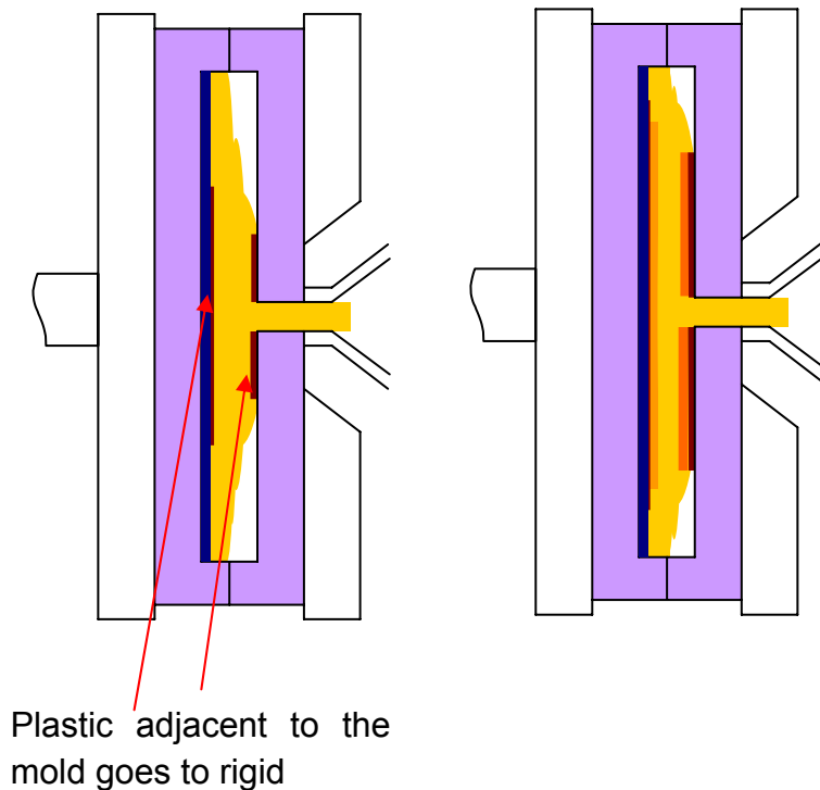
Fig.4-4 Mechanism of the birefringence formation
