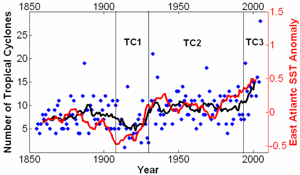
Figure 1. Tropical cyclone occurrence (blue points indicate annual totals and the black line is a 9-y running mean) in the North Atlantic together with East Atlantic SST anomalies for the hurricane season (red line) from 1855-2005. TC1, 2 and 3 refer to climate regimes discussed in the text.
