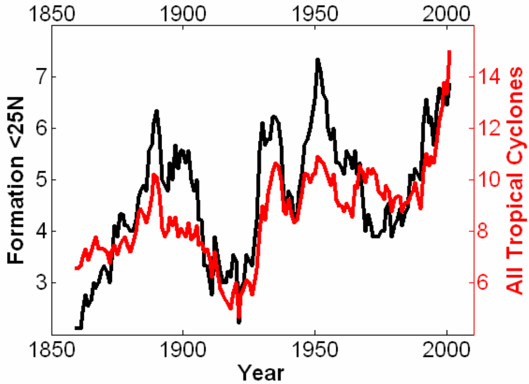
Figure 8. Comparison of the variation in all tropical cyclones (red line) and those forming equatorward of 25°N (black line). All series have been smoothed with a 9-y running mean.
