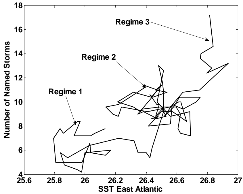
Figure 2: Phase diagram showing relationship between 5-y filtered annual tropical cyclone numbers and SST in the East Atlantic. The three climate regimes discussed in the text are indicated and the changeover between the regimes occurs in the short joining contours. Note that regime 3 has not yet settled into a stable pattern.
