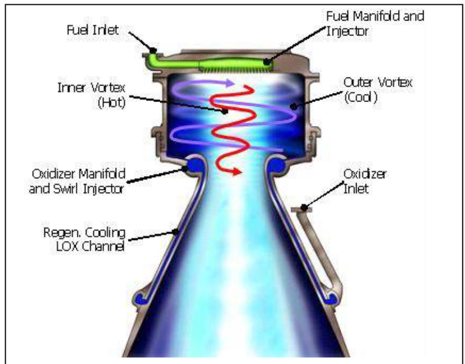
The vortex cooled chamber wall engine contains two co-axial vortices. The oxidizer flowing up from the base forms the outer, insulating vortex, and then spirals in at the head end to form the second vortex that descends to flow out of the engine nozzle. Fuel is injected at the top of this inner combustion vortex. (Source: Orbital Technologies Corporation (ORBITEC™))
