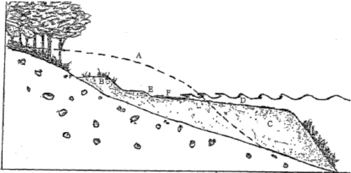
Typical Profile of Lakeshore. A – Original Shoreline, B – Dune, C – Littoral Shelf, D – Ripple Marks On Sand, E – Beach Scarp, F – Glacial Till. Adapted from: Understanding, Living With, and Controlling Shoreline Erosion , Tip of the Mitt Watershed Council, 1995.
