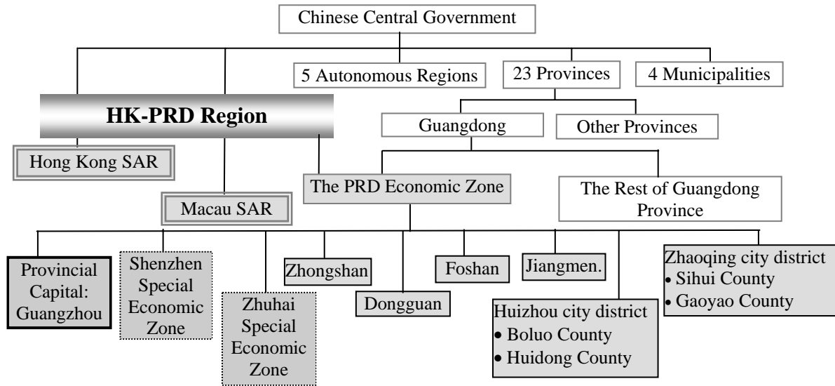
Figure 3. “One environment, multiple systems” in the Hong Kong-PRD region
