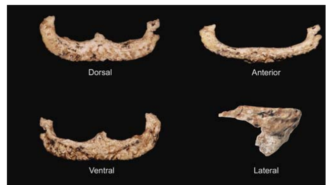
Figure 9. Predentary.
