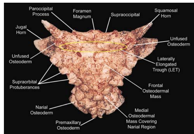
Figure 1. Skull roof.
