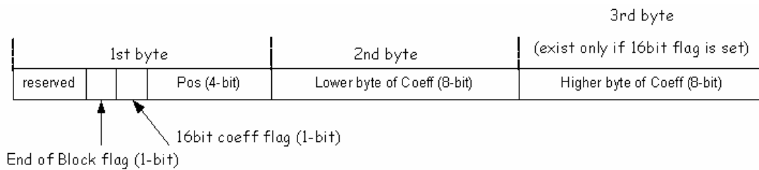
Figure 6-6: Coefficient-Position Pair Buffer Definition
