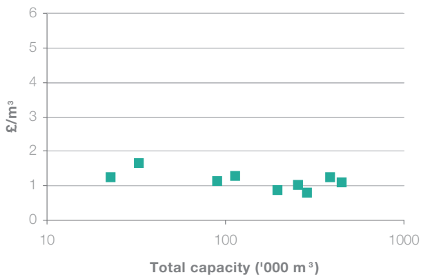
Figure 2 – Clay lined reservoirs – earthworks costs only (2008 prices)
