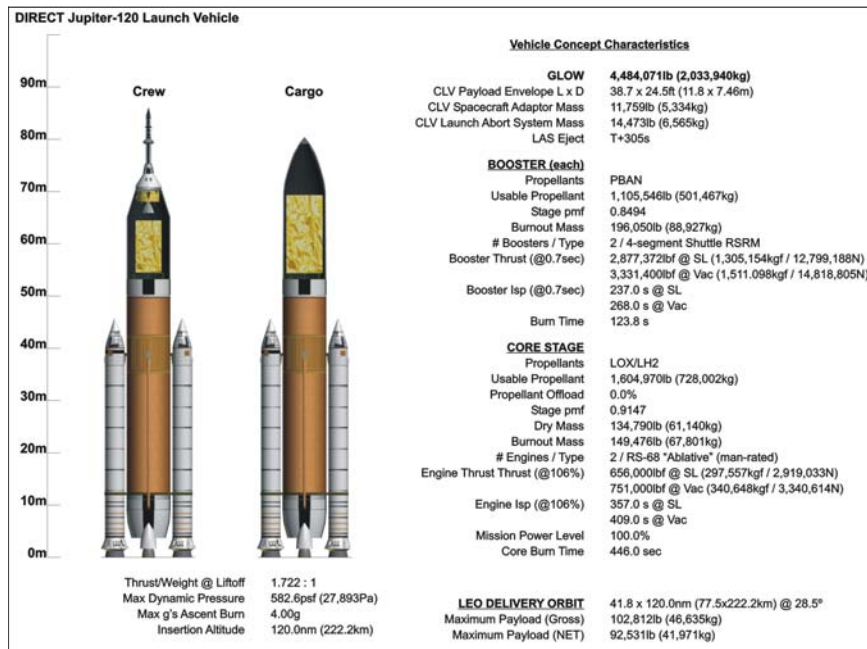
Jupiter 120 Launch vehicle specification. [www.DIRECTLauncher.com]
