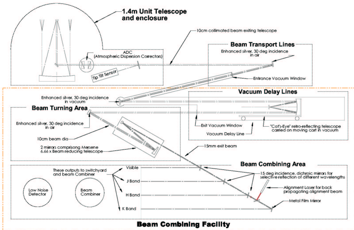
Figure 2. Schematic layout of all components within MROI. Note there are only 15 reflections from primary to detectors.
