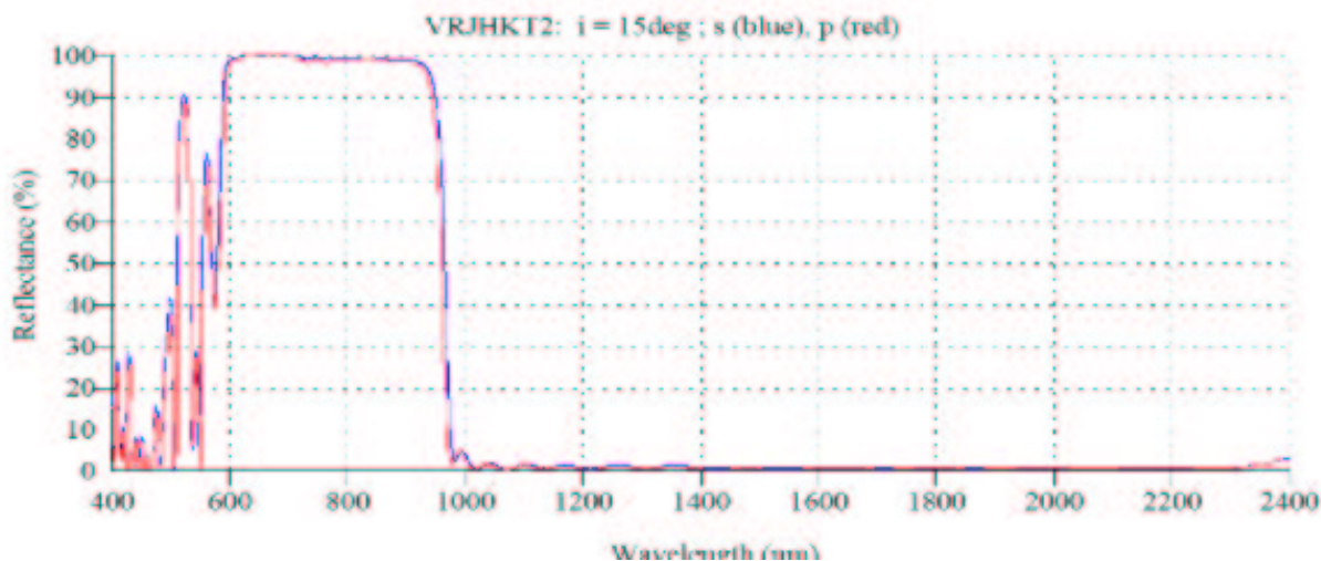
Figure 4. Newly designed multi-layer dichroic coating for MROI (see Hobson & Baldwin 14 ). S and P polarizations overlay nearly exactly, indicating no difference in coating performance due to incident polarization.
