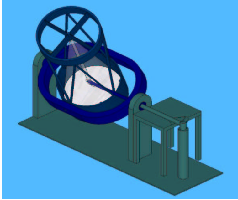
Figure 3. Altitude-altitude telescope design including optical table for the tip-tilt and ADCs.
