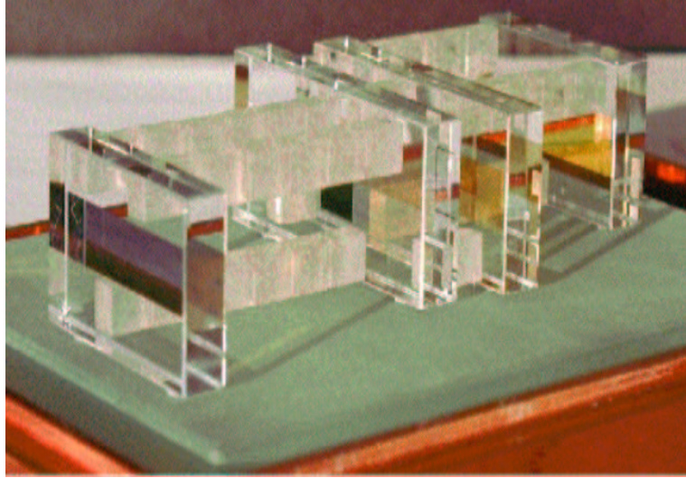
Figure 5. Prototype optically-contacted beam combiner on which MROI will base a hybrid design for an 10-way beam combiner. This beam combiner has a footprint of 10 by 15 cm.
