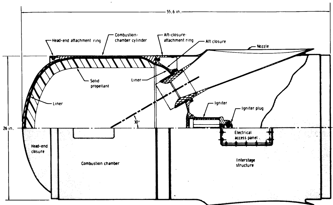
Figure 3. - Tower-jettison motor.
