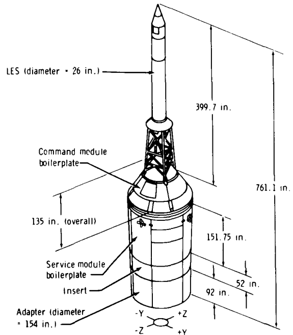
Figure 10. - Apollo BP-13.
