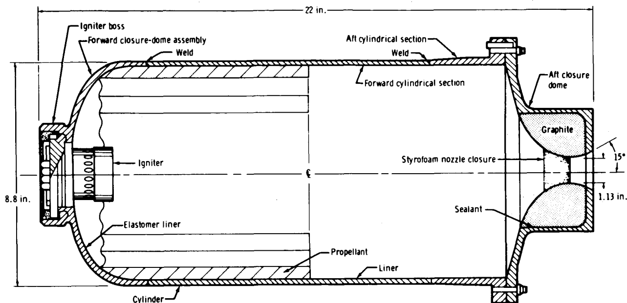
Figure 2. - Pitch-control motor.
