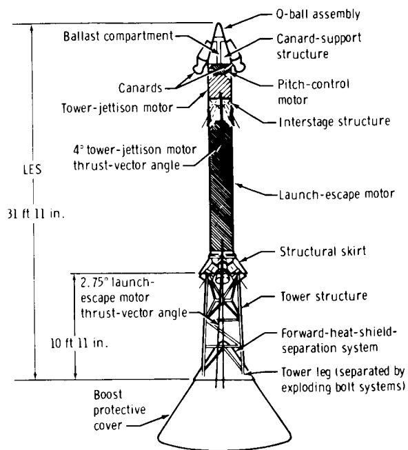
Figure 1. - Apollo launch escape system.
