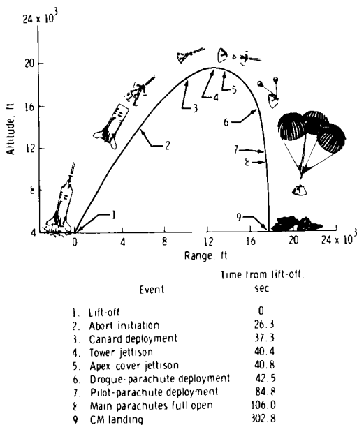
Figure 8. - Major events of Apollo A-003 mission.
