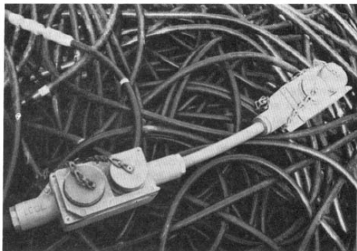
Seismic cable. Note cableheads.
