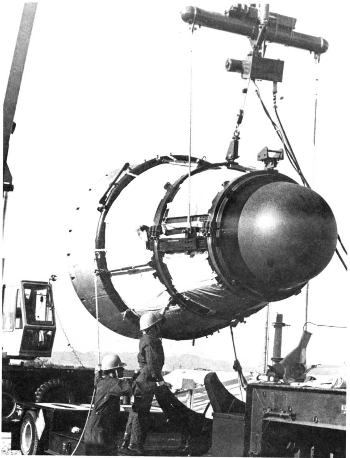
A Titan II Reentry Vehicle belonging to the 390th SMW, Davis-Monthan AFB, AZ, is removed for retirement, May 1984.
