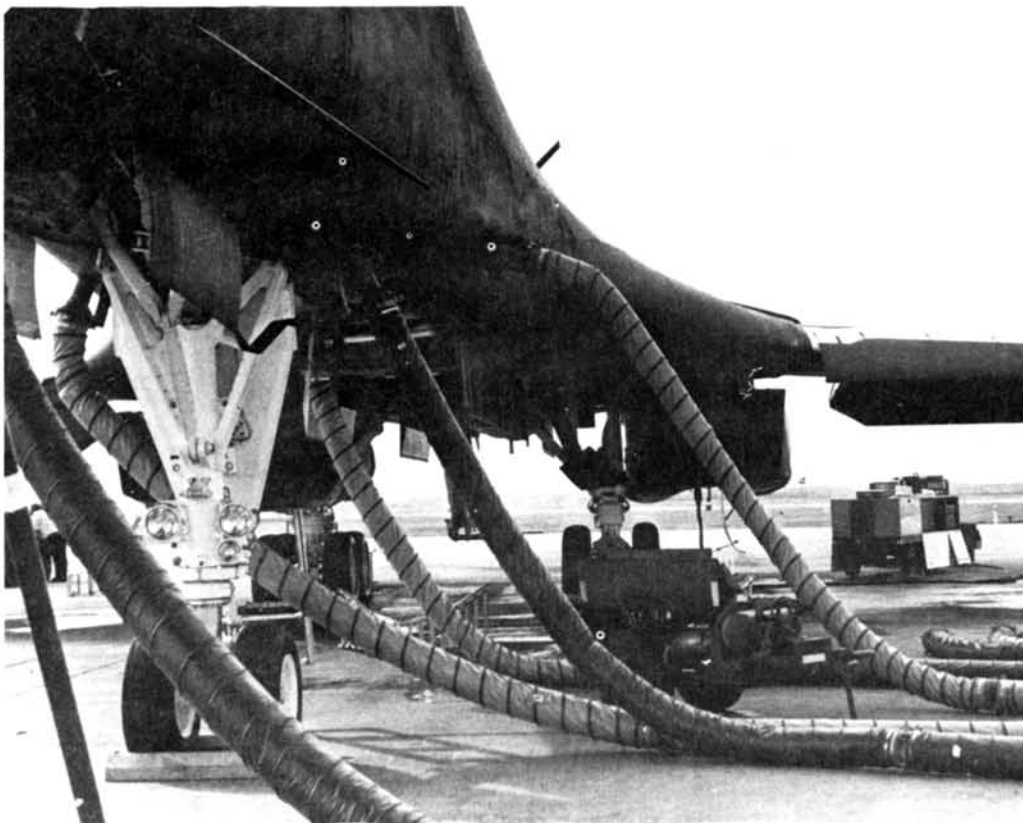
A B-1B undergoing routine maintenance
