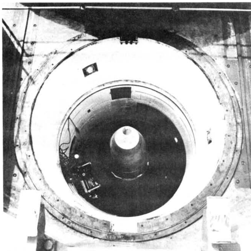
SAC's first multiple warheaded Minuteman III emplaced in launch facility H-2 of the 741st SMS, Minot AFB, ND
