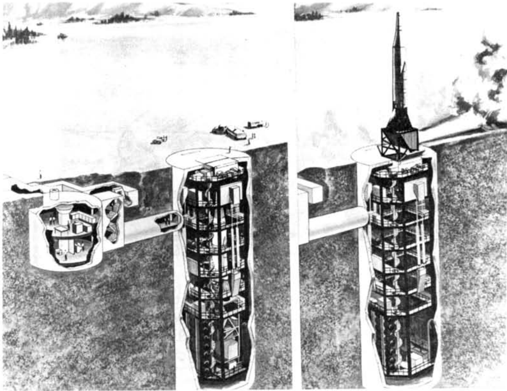
Illustration of an Atlas F Missile Complex
