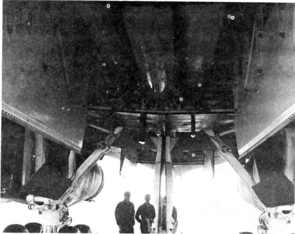
A view of the forward and intermediate weapons bays on the B-1B
