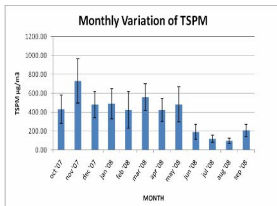
Fig. 5.53: Monthly variation in concentration of TSPM
