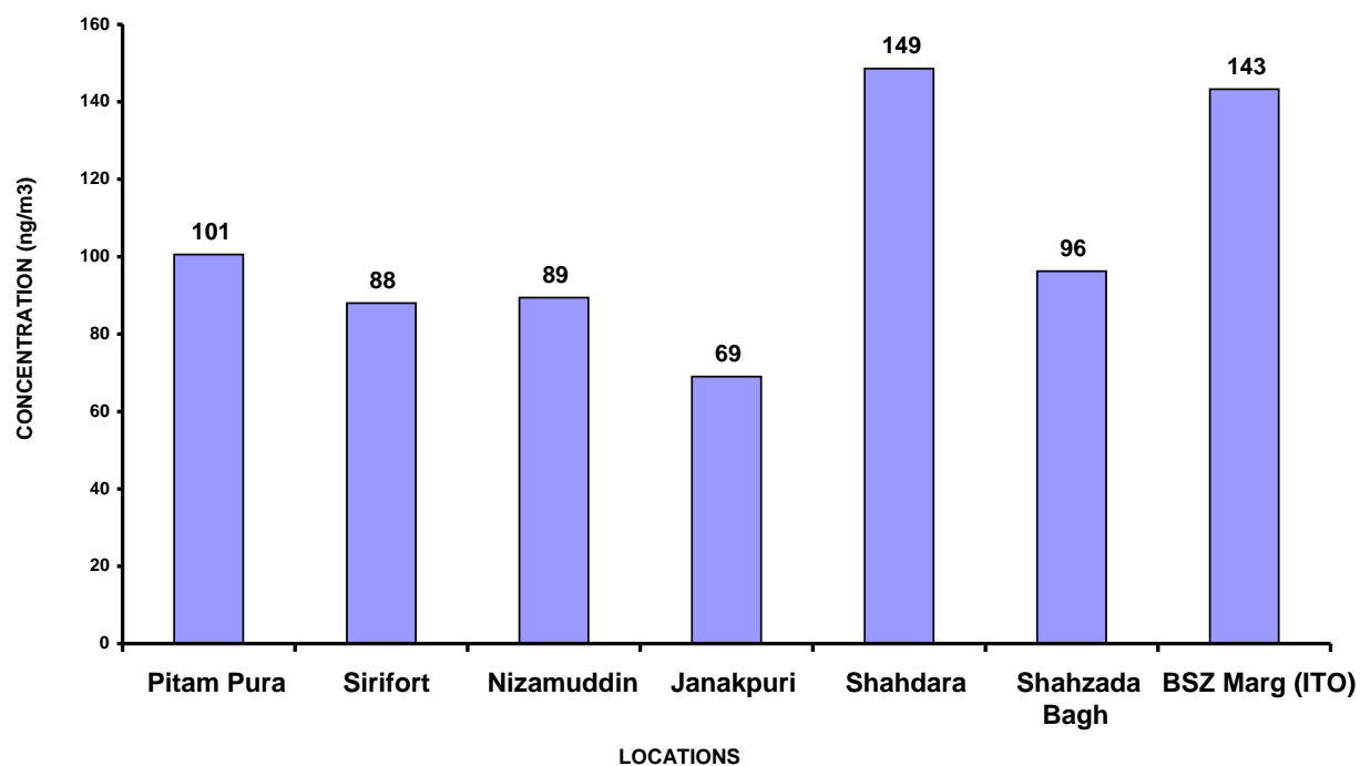
Fig. 5.48: Particulate Lead Concentration in Ambient Air of Delhi (2008)
