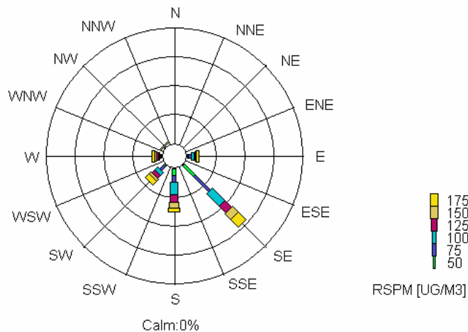
Fig. 5.60: Pollution Dispersion rose at Peenya, Bangalore (March, 2009)
