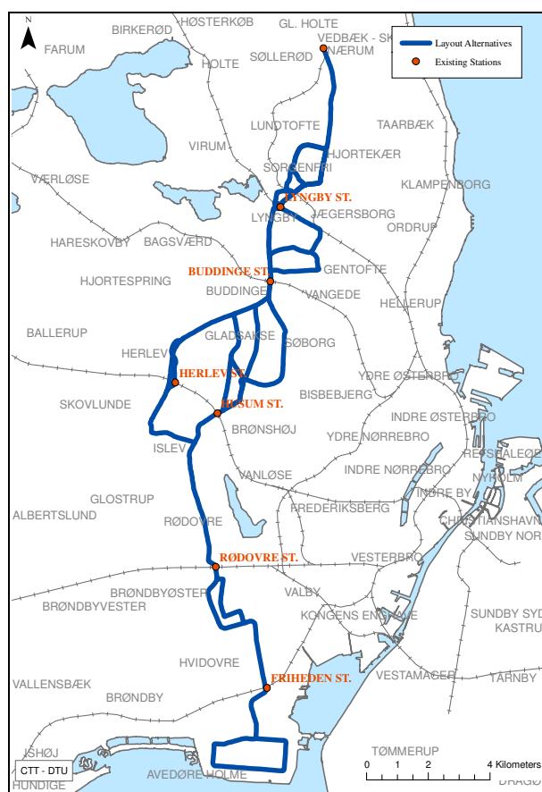
Figure 2 – Alignment alternatives for the Ring 2 1/2 light rail
