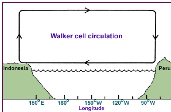
Figure 25. The Walker cell circulation cycle over the Pacific Ocean. The vertical scale is exaggerated, the height of the circulation cell being about 15 km. This atmospheric circulation pattern tends to produce low atmospheric pressure and a warm, moist climate over Indonesia. Atmospheric pressure is relatively high and the climate cool and dry along the coast of northern Peru.
