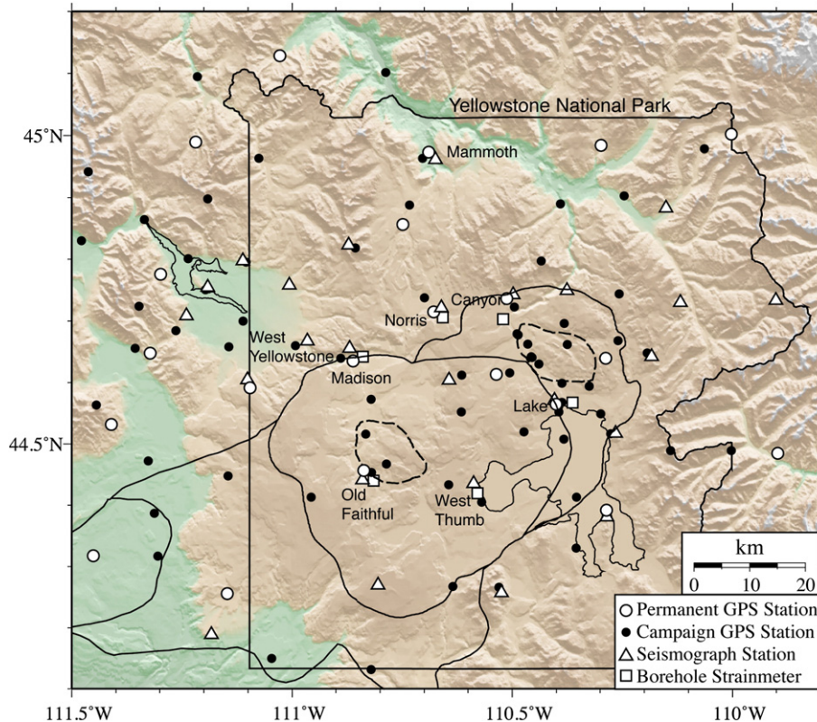
Fig. 7. Station map of Yellowstone National Park and surrounding area showing regional seismic, GPS, and borehole strainmeter networks. Seismic stations consist of broadband and short-period seismometers operated by the University of Utah and the Yellowstone Volcano Observatory. GPS sites include 26 permanent and 90 temporarily occupied (campaign) sites operated by the University of Utah and EarthScope PBO.
