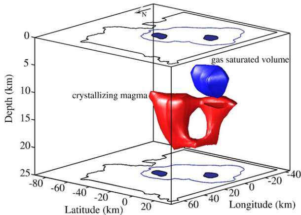
Fig. 10. Isosurfaces of anomalously low ( -1.8\% ) P-wave velocity bodies are determined from local earthquake tomography of the Yellowstone caldera that reveals the Yellowstone magma reservoir. The shallow anomaly plotted in blue is interpreted to be a gas-saturated body. The red anomaly is interpreted to be 5% to 15% partial melt corresponding to a crystallizing magma body that feeds the surface silicic and basaltic magmatism of Yellowstone (from Husen and Smith, 2004). The outline of Yellowstone National Park (black), the Yellowstone caldera (blue), and resurgent domes (dark blue shaded regions) are projected at the top and bottom of the plot.
