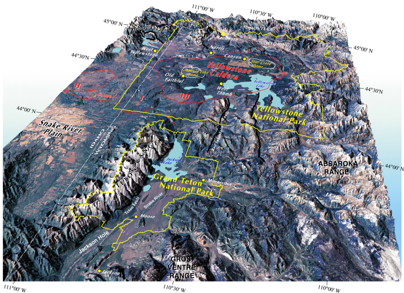
Fig. 3. Space view of Grand Teton and Yellowstone National Parks from LANDSAT satellite imagery overlain on digital elevation data. The caldera occupies a 60 km by 40 km-wide area of central Yellowstone National Park. Park boundaries are shown as yellow lines. Caldera boundaries are outlined in red and labeled I for the 2.05-Ma caldera, II for the 1.3-Ma Henrys Fork Caldera, and III for the 0.64-Ma Yellowstone Caldera. Resurgent domes are outlined in white. Local place names are marked with yellow circles. Modified image from Smith and Siegel (2000).
