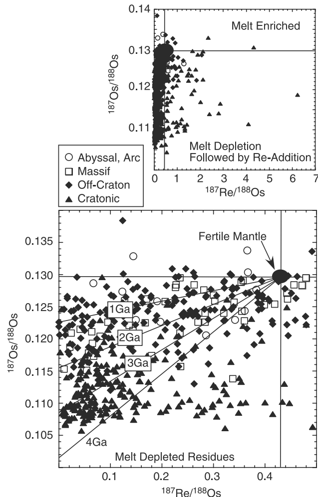
Figure 8. Re-Os isochron diagram showing the data for various types of samples of continental lithospheric mantle. The vertical and horizontal lines in Figure 8 pass through an estimate of the average Re-Os characteristics of the fertile mantle [Meisel et al. , 1996] and divide the plot into quadrants that can be reached through single-stage melt depletion (bottom left) and corresponding melts (top right) from average mantle. Data can only reach the top left and bottom right quadrants through an additional chemical fractionation event; for example, the scattering of points into the bottom right quadrant most likely reflects depleted xenoliths that have interacted with their transporting magma thereby raising their Re/Os ratio but not significantly changing their Os isotopic composition. Sloped lines in Figure 8 reflect data arrays expected for single-stage melt residues of 1, 2, 3, and 4 Ga age. Data are from Walker et al. [1989], Reisberg et al. [1991], Carlson and Irving [1994], D. G. Pearson et al. [1995a, 1995b, 1995c, 1998b, 1999, 2002, 2004], N. J. Pearson et al. [2002], Reisberg and Lorand [1995], McBride et al. [1996], Meisel et al. [1996, 2001], Handler et al. [1997, 2003], Carlson et al. [1999a, 1999b], Chesley et al. [1999], Menzies et al. [1999], Ruiz et al. [1999], Burton et al. [2000], Lee et al. [2000], Peslier et al. [2000a, 2000b], Snow et al. [2000], Becker et al. [2001], Hanghoj et al. [2001], Irvine et al. [2001, 2003], Lee et al. [2001], Richardson et al. [2001], Alard et al. [2002], Gao et al. [2002a], Griffin et al. [2002], Schmidt and Snow [2002], Wang et al. [2003], Westerlund et al. [2003], Wu et al. [2003], and Carlson and Moore [2004].
