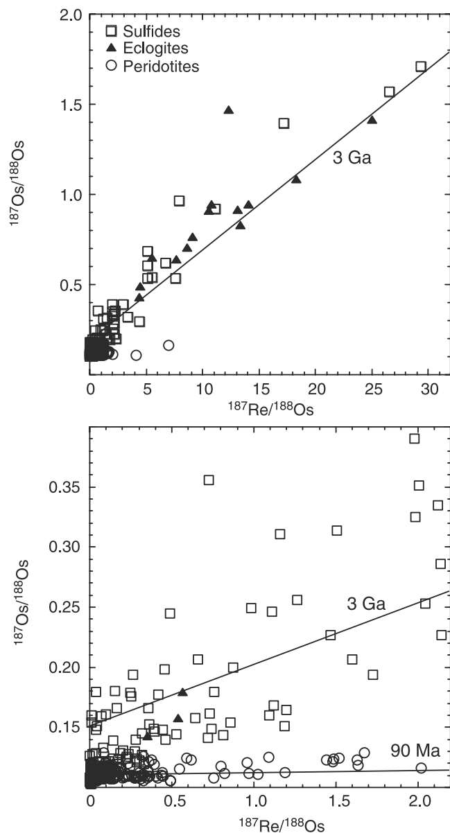
Figure 9. Re-Os isochron diagram for whole rock peridotites (circles), sulfides from Kaapvaal mantle peridotites (squares), and eclogites (triangles) from the cratonic mantle. Lines with slope corresponding to 90 Ma and 3 Ga age are shown for reference. Data for whole rock peridotites are from the sources given in Figure 8; eclogite data are from Menzies et al. [2003] and Pearson et al. [1995c]; Kaapvaal sulfide data are from Griffin et al. [2004].
