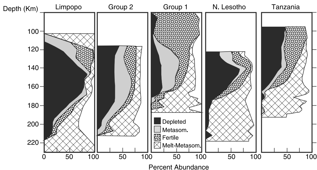
Figure 13. Relative abundance of different chemical types in the African lithospheric mantle as deduced from the analysis of garnet concentrates from the kimberlite groups shown by the labels at the top of each plot. The plots are arranged in age progression of the kimberlite localities from (left) oldest to (right) youngest. Figure modified from that presented by Griffin et al. [2003], reprinted with permission from Elsevier.
