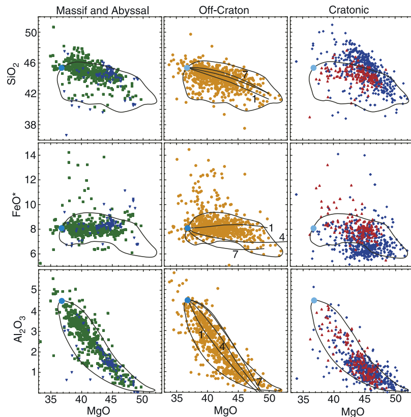
Figure 6. Major element ranges observed for peridotites from a variety of tectonic settings including (left) ocean basins (dark blue points) and mantle sections tectonically obducted onto continental crust (massif peridotites (green points)), (middle) peridotite xenoliths (primarily spinel peridotites) erupted in tectonomagmatically active areas away from cratons, and (right) peridotite xenoliths carried by kimberlites erupting through both Archean and middle to Early Proterozoic crust. In the right column the blue points are for low-T peridotites, and the red points are for high-T samples. The field shown on all plots outlines the majority of the data for off-craton peridotite xenoliths to serve as a reference. The large light blue dot in all plots is an estimate of fertile mantle composition. Lines emanating from fertile mantle in the center column plots show the expected composition of residues of partial melting occurring at 1, 4, and 7 GPa [Walter, 1999, 2003]. Peridotite data are from the compilation of McDonough [1990].
