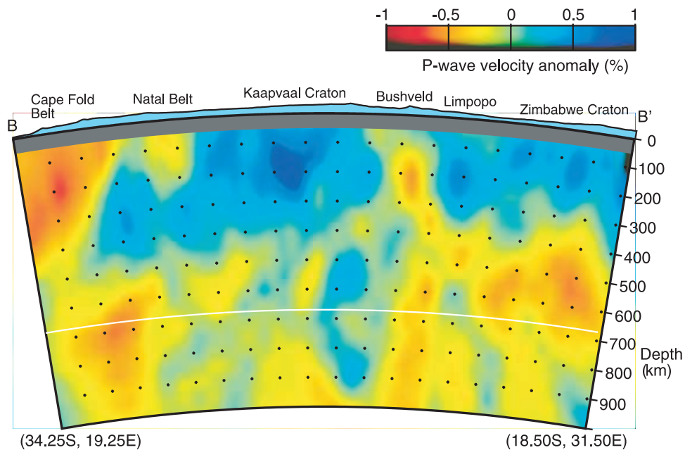
Figure 3. Cross section showing the P wave velocity variation in the upper mantle of southern Africa [James et al. , 2001]. The cross section runs from SW to NE beginning in Cape Town (B) and extending into central Zimbabwe (B'). The light blue band at the top shows vertically exaggerated surface topography. Along the top of the cross section are listed the major crustal terrains encountered from the circa 600–700 Ma Cape Fold Belt, through the mid-Proterozoic Namaqua-Natal Belt, into the Archean Kaapvaal and Zimbabwe cratons. Also shown are the surface location of the 2.0 Ga Bushveld igneous intrusion into the Archean crust of the Kaapvaal craton and the Limpopo Belt, a zone of late Archean collision between the Kaapvaal and Zimbabwe cratons. Zones of seismically fast mantle are largely restricted to beneath the Archean crust and extend to depths of at least 250–300 km.
