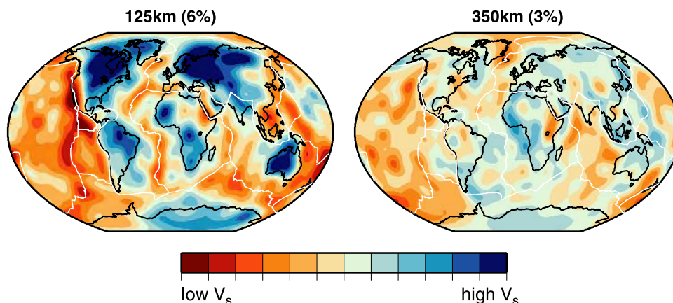
Figure 1. Map of shear wave velocity variation in the mantle at depths of (left) 125 and (right) 350 km. The total range in velocities at 125 km is \pm 6\% and \pm 3\% at 350 km depth. White lines are plate boundaries; continents are outlined in black. At 125 km depth the continent-ocean distinction is clearly visible in the high (blue) seismic velocities characteristic of continental lithospheric mantle. By 350 km depth the correlation between continents and high V_s is no longer clear. Figure produced by J. Ritsema with data from the s20rts model of Ritsema et al. [2004].
