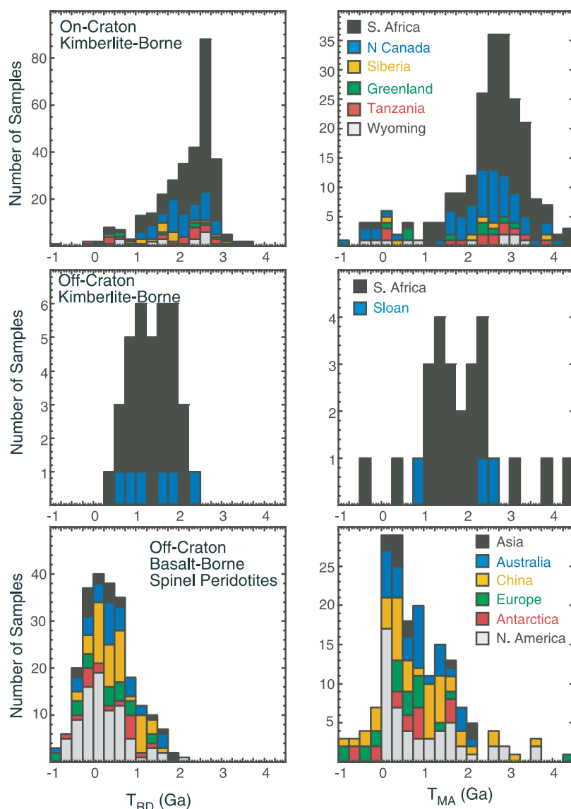
Figure 10. Re-depletion ( T_{RD} ) and conventional Re-Os mantle ( T_{MA} ) model ages for peridotite xenoliths from the continental mantle calculated with respect to the primitive mantle Re-Os parameters given by Meisel et al. [2001]. The data are grouped according to geologic setting of the eruptive host of the xenoliths. (top) Xenoliths carried by kimberlites erupting through Archean crust. (middle) Kimberlite-borne xenoliths erupting through long stable Proterozoic crustal sections. (bottom) Basalt-borne xenoliths erupting in tectonomagmatically active areas away from cratons. Data sources are as referenced for Figure 8.
