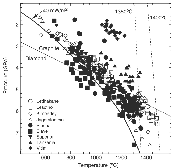
Figure 4. Mineral thermobarometry results for mantle xenoliths from a variety of continental areas [Ionov et al., 1993; Rudnick and Nyblade, 1999]. Curve shows a 40 \text{ mW/m}^2 conductive geotherm assuming that the lithospheric mantle has no internal heat production [Pollack and Chapman, 1977]. The straight line is the diamond-graphite phase boundary [Kennedy and Kennedy, 1976], and the dotted and dashed lines show the position of adiabats for potential temperatures of 1350^\circ\text{C} and 1400^\circ\text{C} , respectively [Rudnick and Nyblade, 1999].
