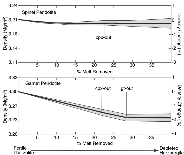
Figure 5. Density change in spinel and garnet peridotite at room temperature and pressure due to melt removal. The bold line in plot shows the density change as a function of the percentage of melt removed, with the shaded band showing the error margin of the density calculation. Also indicated on the plots is the percentage of melting where clinopyroxene (cpx-out) and garnet (gt-out) are completely consumed. Figure modified from Schutt and Leshner (submitted manuscript, 2004).
