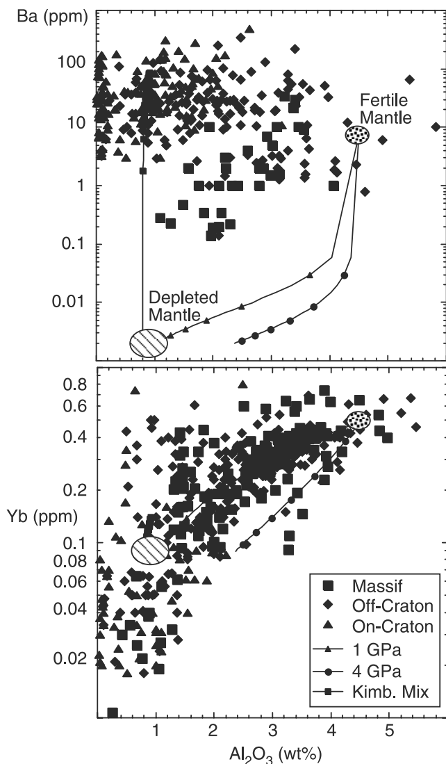
Figure 7. Comparison of the observed concentration of a highly (Ba) and moderately (Yb) incompatible trace element versus \text{Al}_2\text{O}_3 concentration in mantle peridotites from various tectonic settings. Lines denoted by triangles (1 GPa) and circles (4 GPa) show the compositional variation expected for partial melting residues [Walter, 1999] starting from an estimate of fertile mantle shown by the smaller oval. Each point along these lines indicates 10% increments in the amount of partial melt removed. The line marked by the squares shows the mixing trajectory between a residue of high-degree partial melting (large oval) and a primary kimberlitic magma [Le Roex et al., 2003]. Points along these lines reflect 0.5% increments in kimberlite addition to a total of 10% kimberlite, with 90% depleted peridotite. Peridotite data are from the compilation of McDonough [1990].
