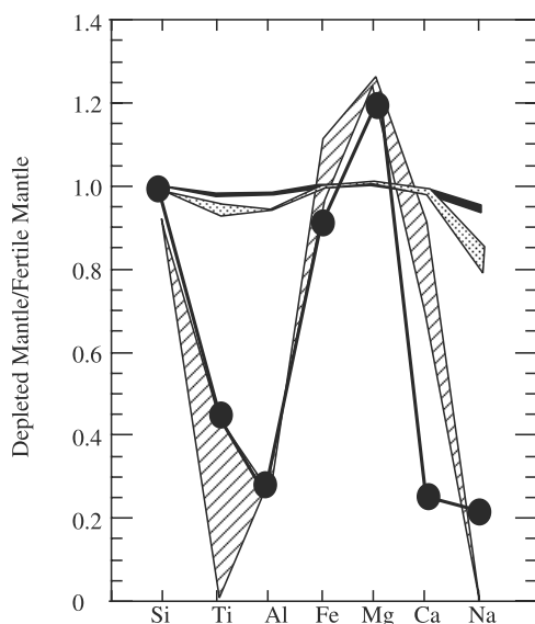
Figure 12. Fertile mantle normalized major element abundances of mantle depleted by the extraction of the current volume of continental crust using extreme estimates for the average composition of the continental crust [Weaver and Tarney, 1984; Taylor and McLennan, 1985]. The amount of chemical fractionation in the mantle residue depends on the amount of mantle affected by continent extraction as shown by the solid (100% by mass of the mantle affected), dotted (30% by mass of the mantle affected), and hatched (2% by mass of the mantle affected) areas. Dots show the composition of average continental garnet peridotite from McDonough [1990].
