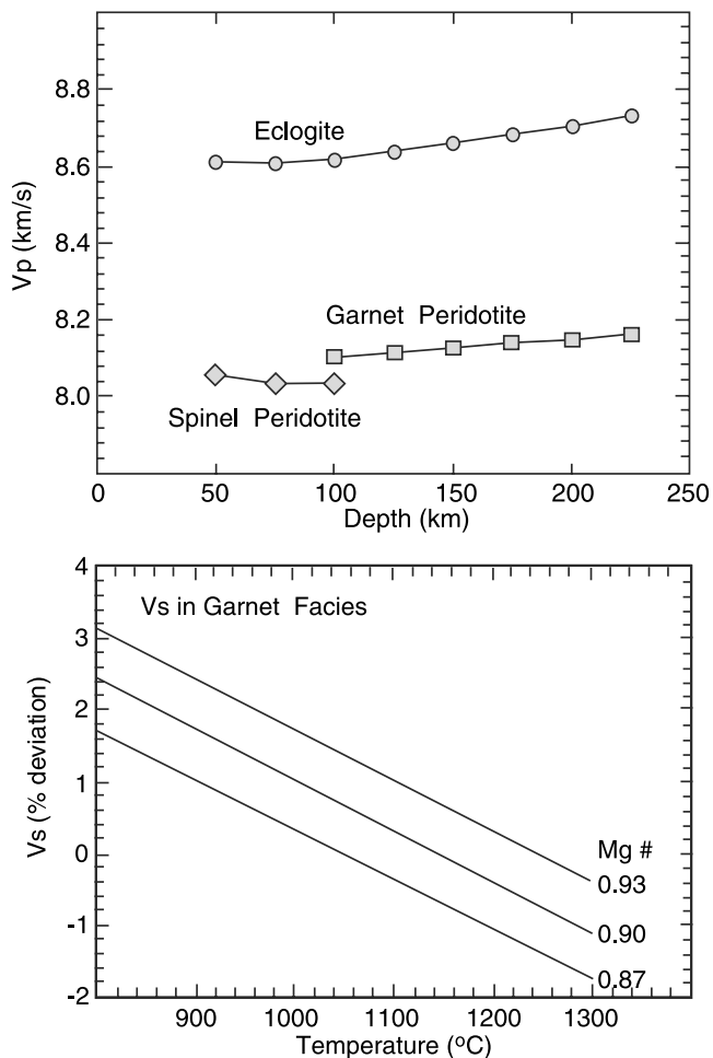
Figure 2. (top) Range of calculated compressional wave velocities ( V_p ) for hypothetical mantle eclogite and fertile peridotite compositions based on the Kaapvaal craton geotherm determined by xenolith thermobarometry [James et al. , 2004]. (bottom) Relationship between shear wave velocity ( V_s ) and temperature in garnet peridotite with different magnesium numbers ( Mg\# = Mg/(Mg + Fe) in the whole rock sample) [after Lee, 2003].
