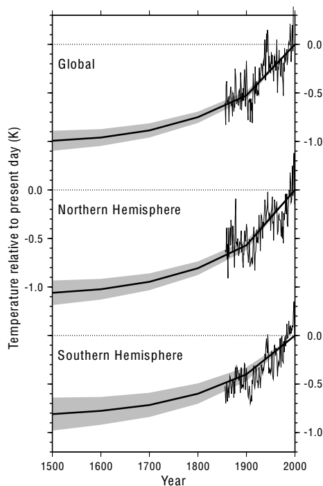
Figure 2 Global and hemispheric averages of GST history over the past five centuries. Shaded areas represent 6 standard errors about the mean. Superimposed are the corresponding series of instrumental surface air temperatures (SAT) 6 . Because the geothermal reconstruction is the concatenation of century-long trends, and the SAT anomaly series are referenced to the mean over the period 1961–90, we have shifted the SAT series along the temperature axis to enable an easy comparison of their respective trends. The SAT records have been shifted –0.20 K for the global series, –0.28 K for the Northern Hemisphere and –0.13 K for the Southern Hemisphere.
