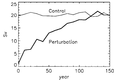
Figure 1. Timeseries of the strength of the THC in the perturbation run (heavy) and control run (light). Shown are decadal mean values of the meridional stream function in the Atlantic at 48^{\circ} N, at 666 m depth.
