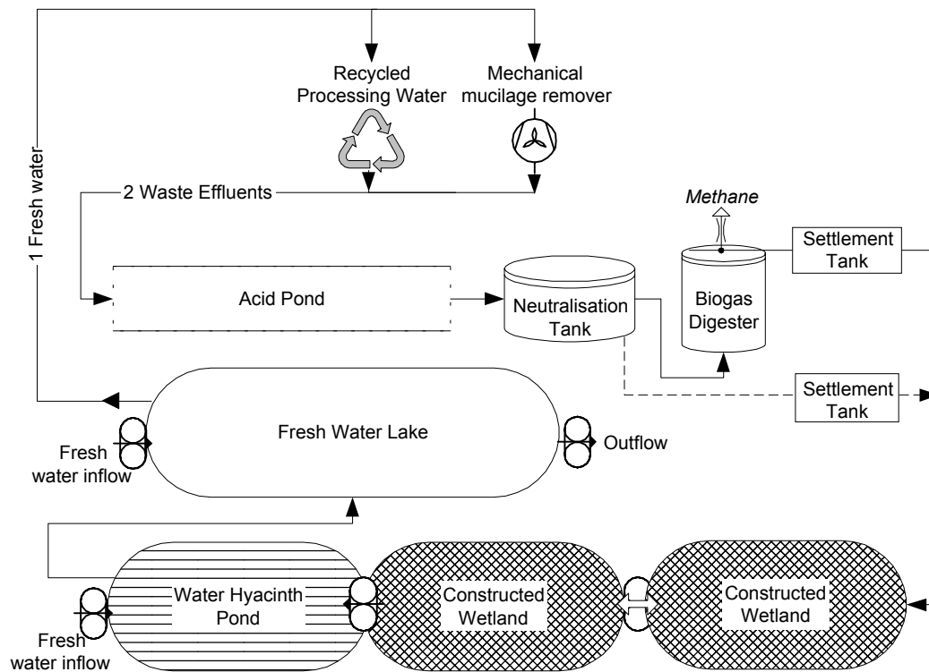
Waste water treatment setup, Khe Sanh, Quang Tri
