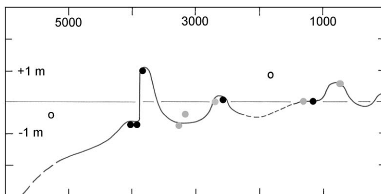
Fig. 1. Sea level curve for the last 5000 years for the Maldives. Black dots=past sea level positions dated by radiocarbon (AMS), grey dots=dates by Woodroffe (1992) with uncertain relation to sea level, open circles=dates by Woodroffe (1992) without closer relation to a former sea level. The sea level curve is oscillating with four levels above the present level; +1.1–1.2 m at 3900 BP, +0.1–0.2 m at 2700 BP, +0.5–0.6 m at 1000–800 BP and +0.2–0.3 m at AD 1900–1970. The islands have been inhabited, at least, since 1500 BP.
